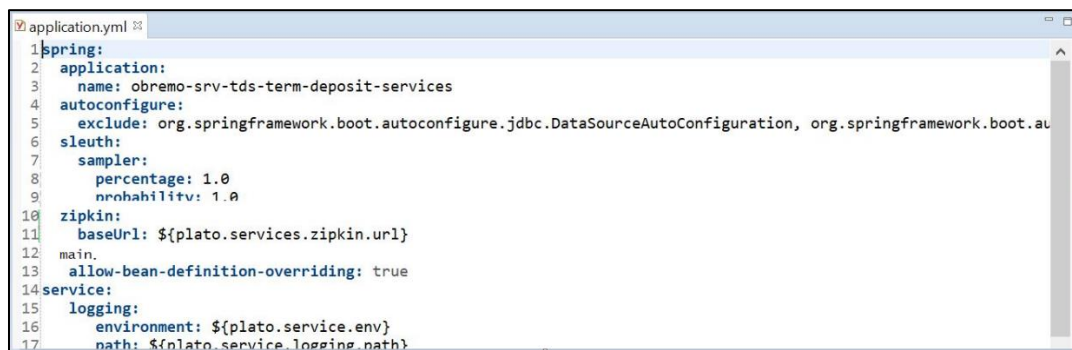
Figure 9: Application.yml File
