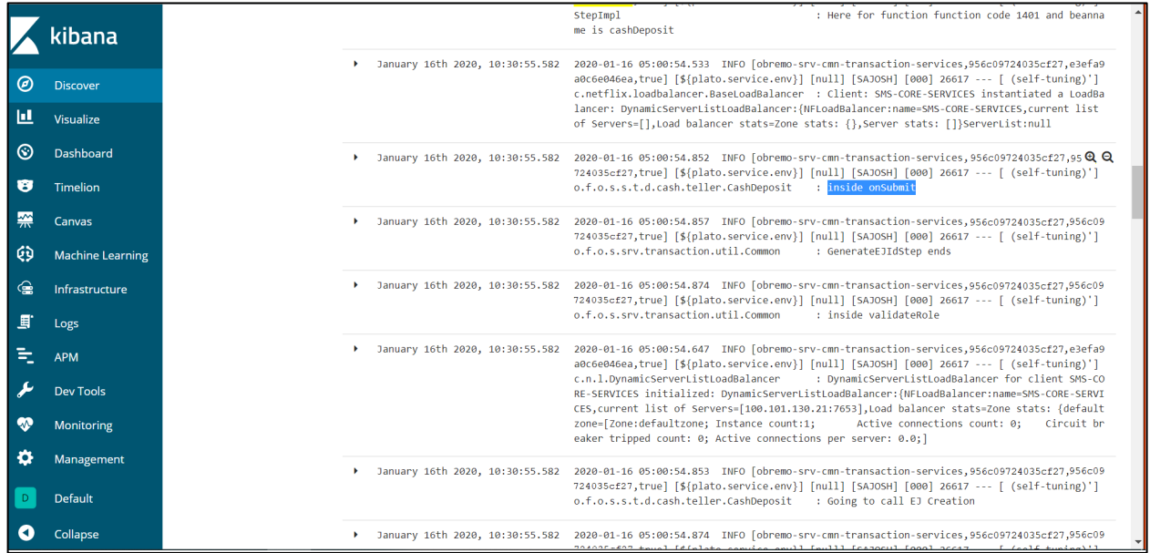
Figure 14: Accessing Kibana
