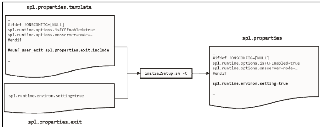
Figure 35: Include Files
