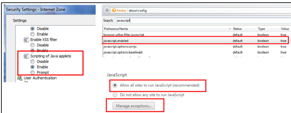
Figure 16: Javascript Settings
