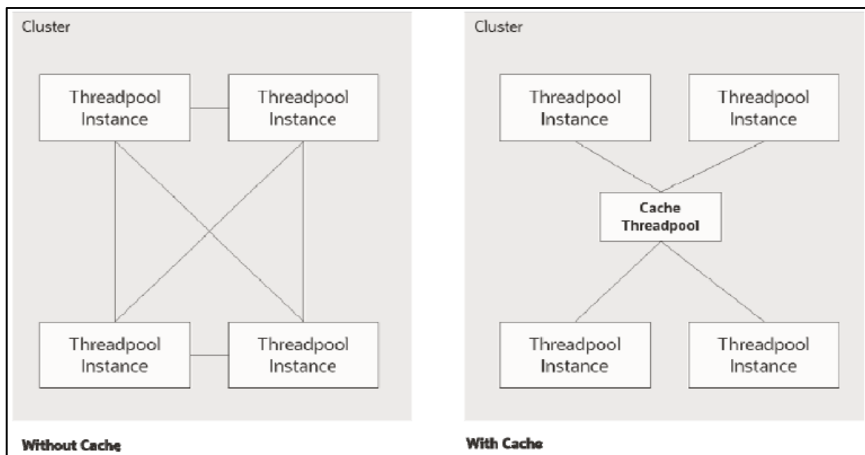
Figure 32: Cache Architecture
