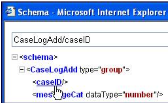
Figure 4: Schema Viewer
