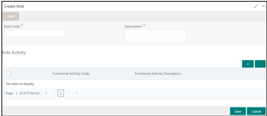
Figure 1.2: Create Role
