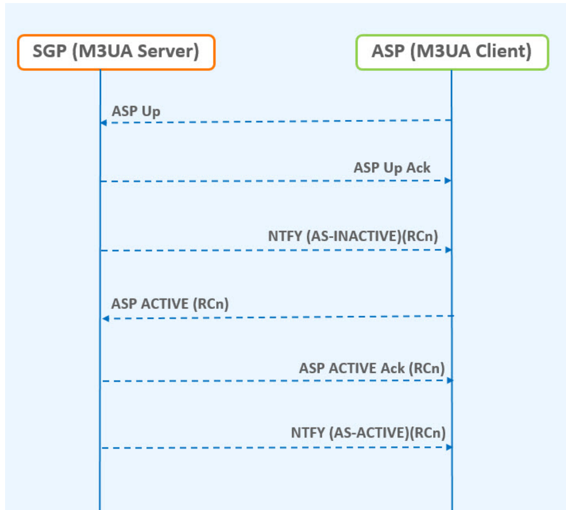
Figure 2-3 Message Flow for ASP - M3UA Client
