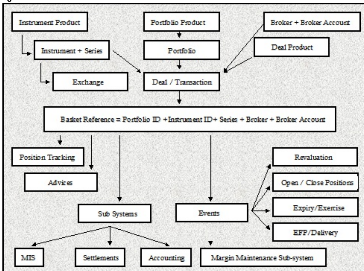
Figure 2.1: ETD Work-flow
