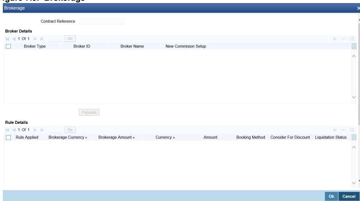
Figure 7.8: Brokerage
