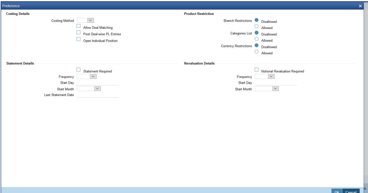
Figure 6.4: Preferences
