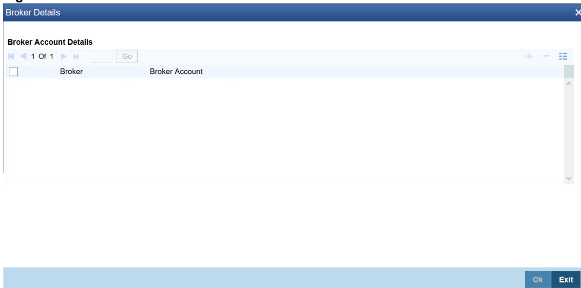
Figure 6.14: Broker Details
