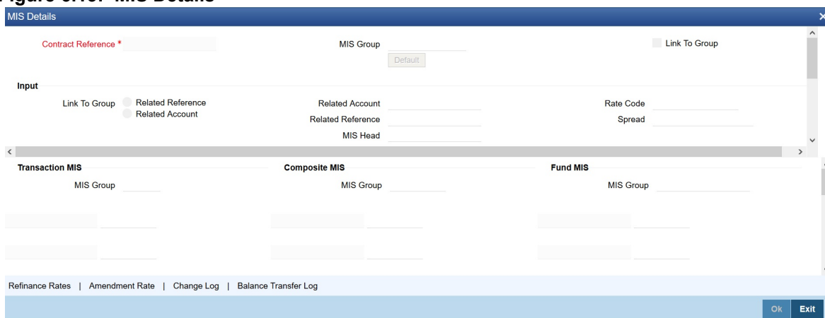
Figure 6.13: MIS Details
