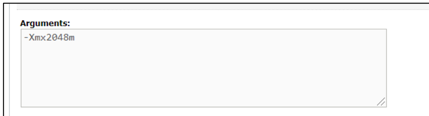
Figure 13: Memory Requirements
