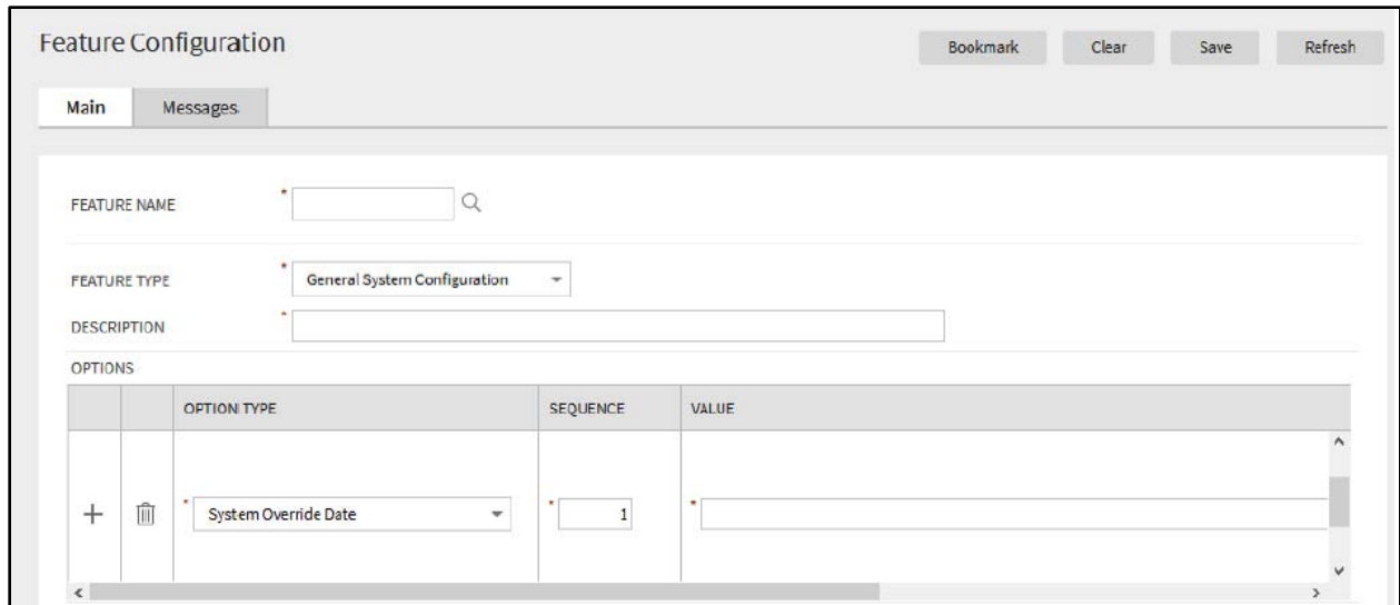
Figure 38: Feature Configuration
