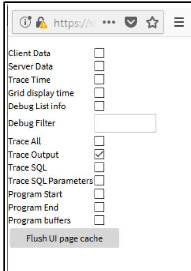
Figure 7: Debug Controls
