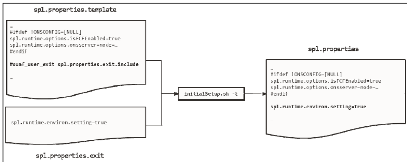
Figure 35: Include Files
