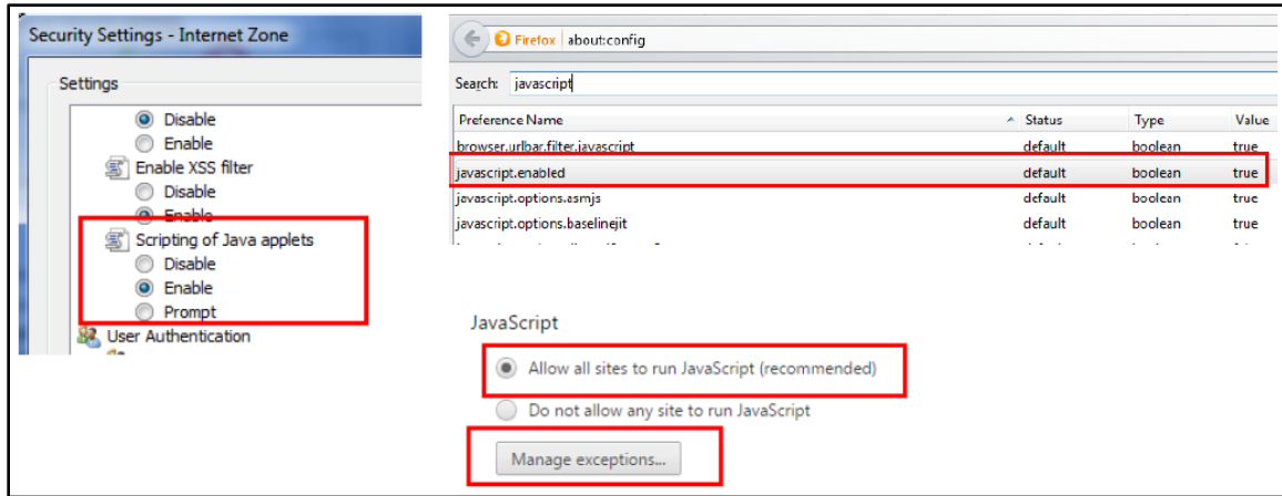
Figure 16: Javascript Settings
