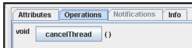
Figure 42: CancelThread Example
