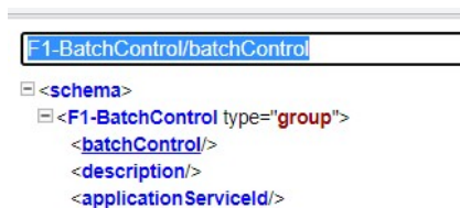
Figure 4: Schema Viewer
