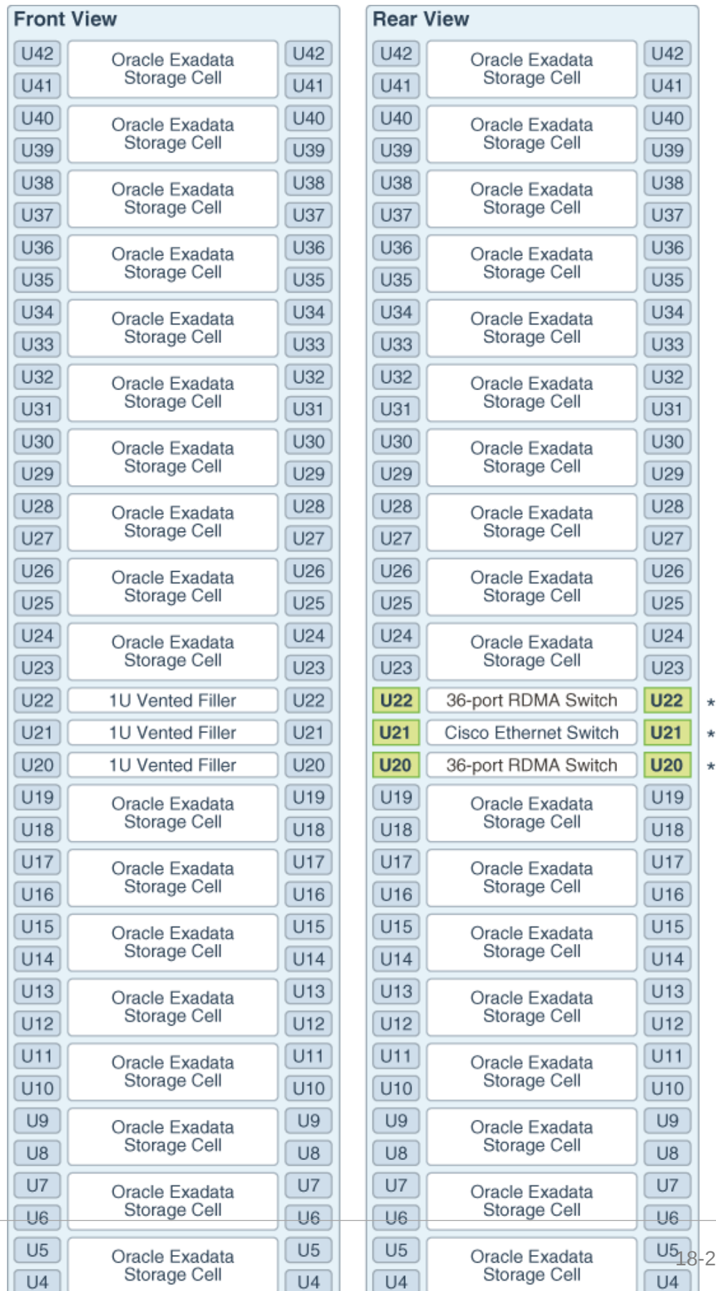
Figure 18-1 Rack Layout of Oracle Exadata Storage Expansion Rack X9M-2
