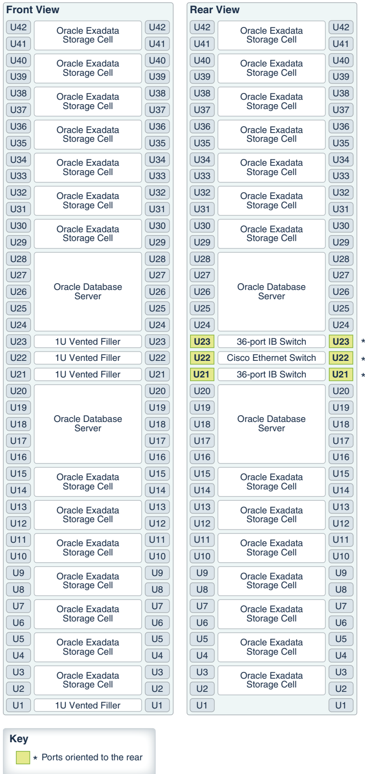
Figure 13-2 Rack Layout of Oracle Exadata Database Machine X8-8 and X7-8
