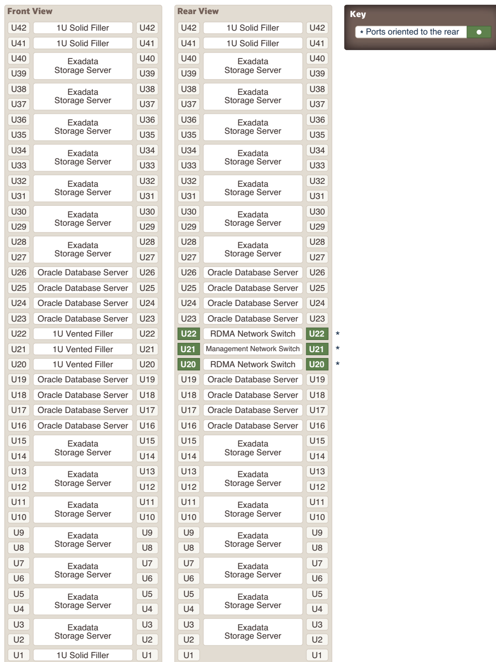
Figure 12-1 Rack Layout of Exadata Database Machine X8M-2 Full Rack
