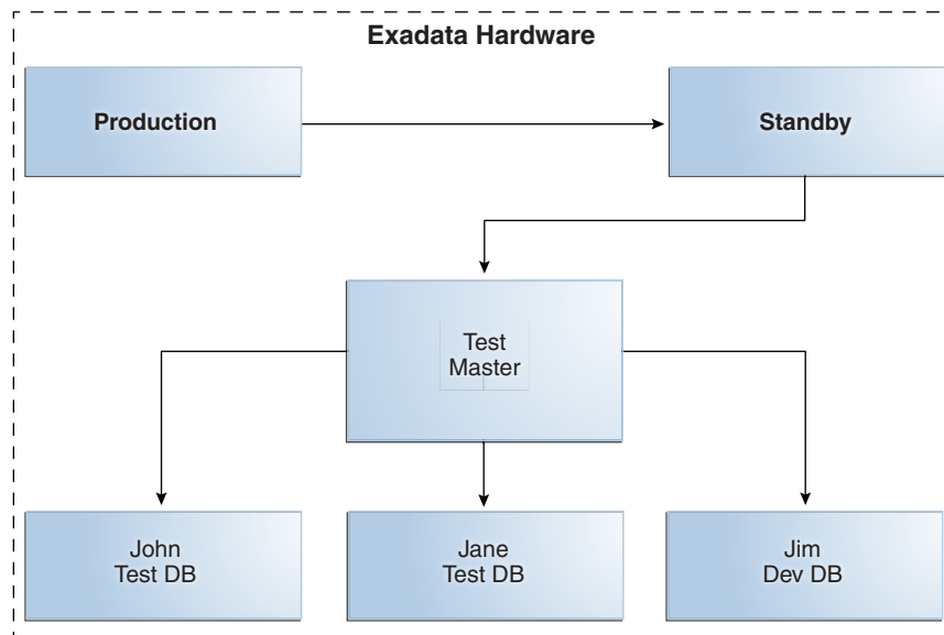
Figure 10-4 An Exadata Environment with 3 Exadata Snapshots from the Same Test Master
