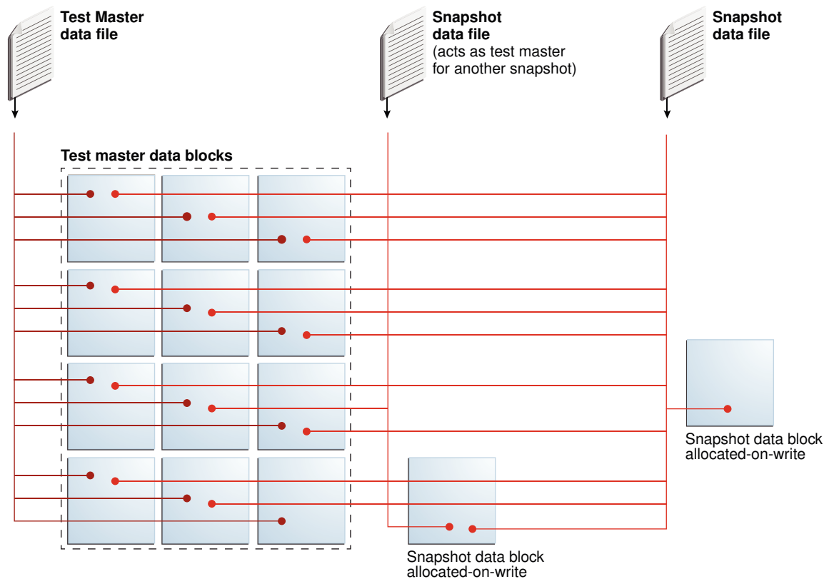
Figure 10-8 Allocation of Blocks in Hierarchical Snapshot Databases
