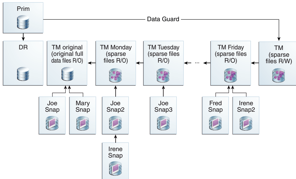
Figure 10-18 Potential Future Configuration
