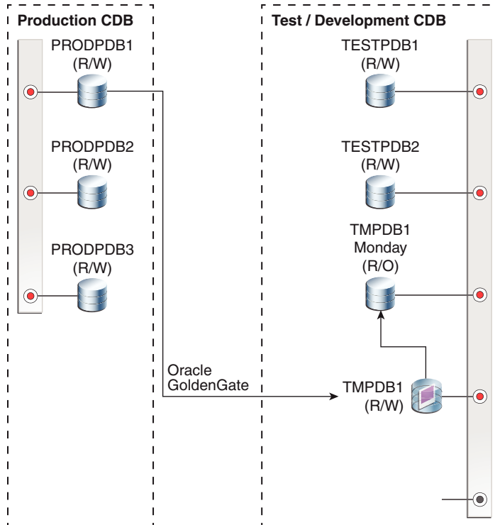
Figure 10-20 TMPDB1 Created From TMPDB1_MONDAY
