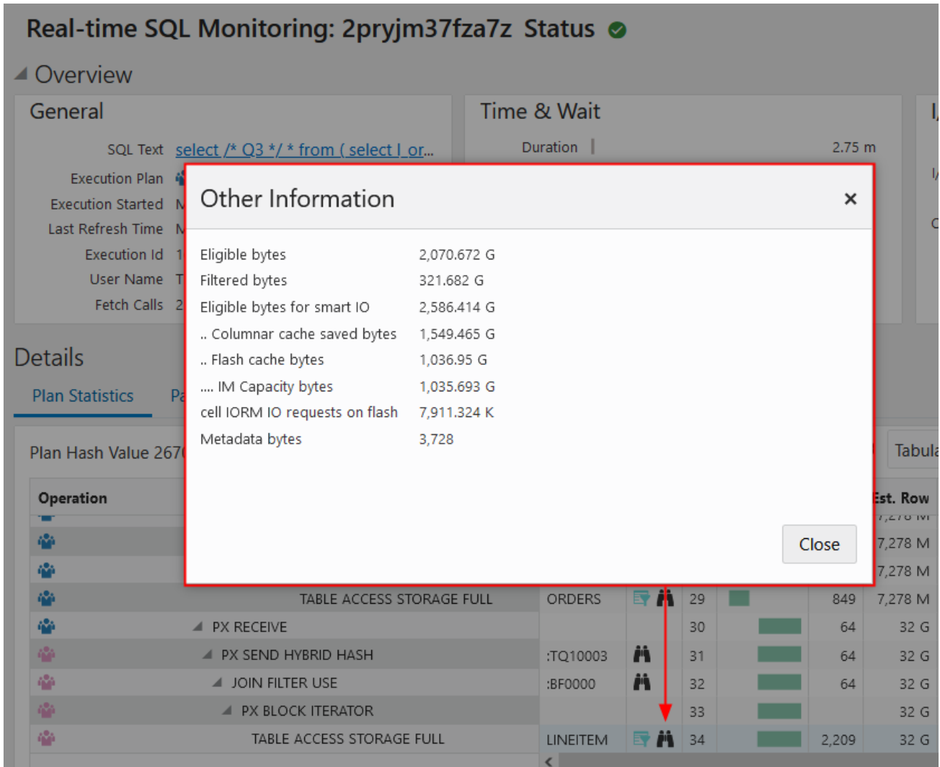
Figure 7-18 SQL Monitor Report: Smart I/O Row Source Statistics
