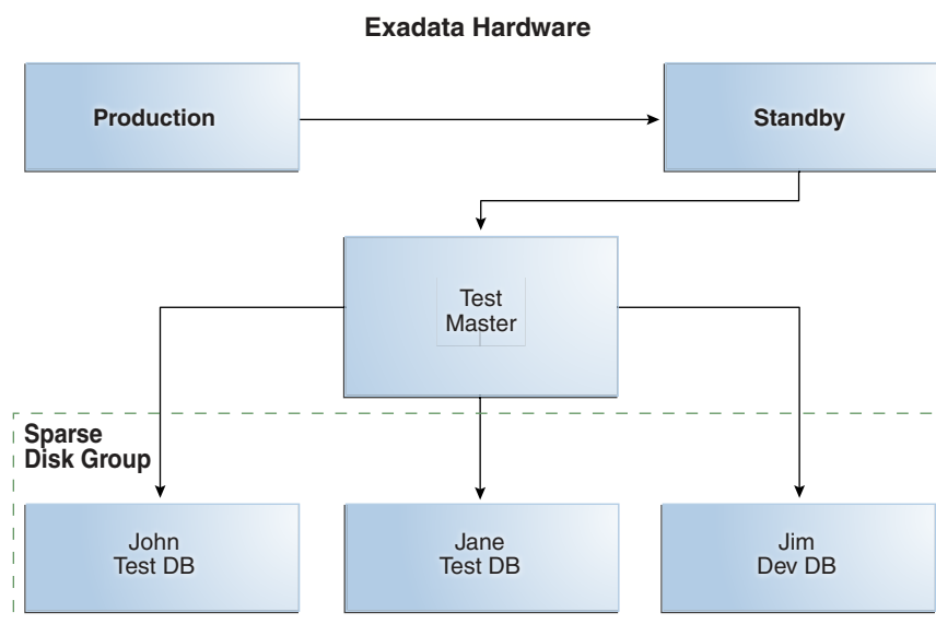
Figure 10-10 Sparse Disk Group Contains Exadata Snapshots
