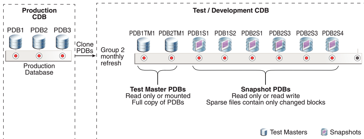
Figure 10-5 Exadata Snapshot PDBs
