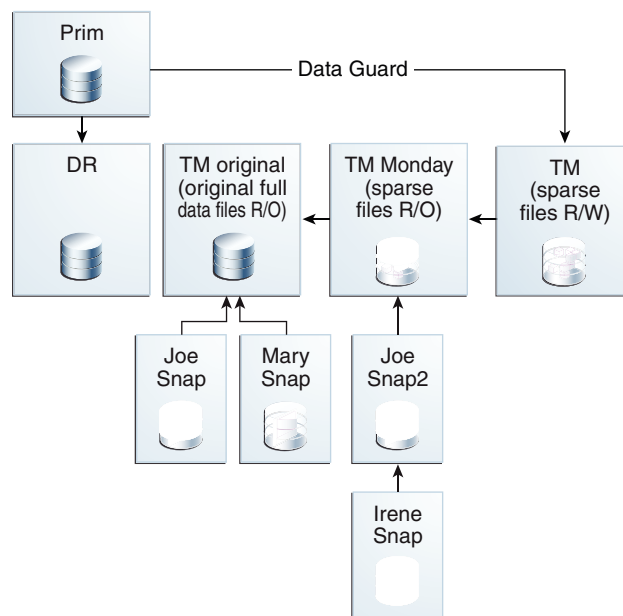
Figure 10-17 Configuration After Repeating the Process
