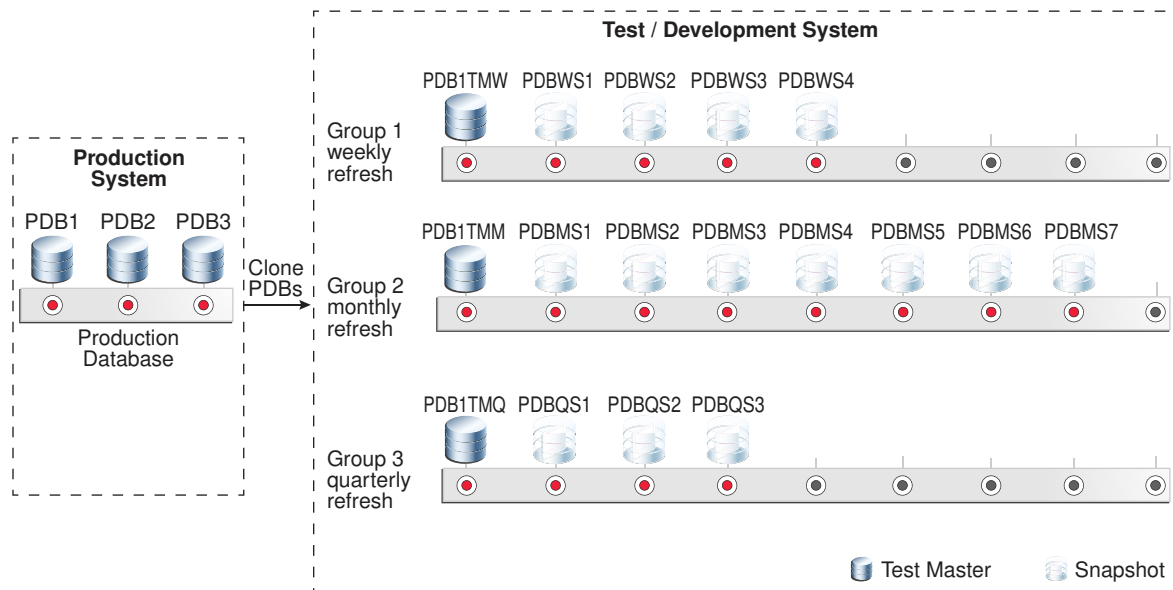
Figure 10-11 Three Developer Groups for PDB1, Each With a Different Refresh Cycle
