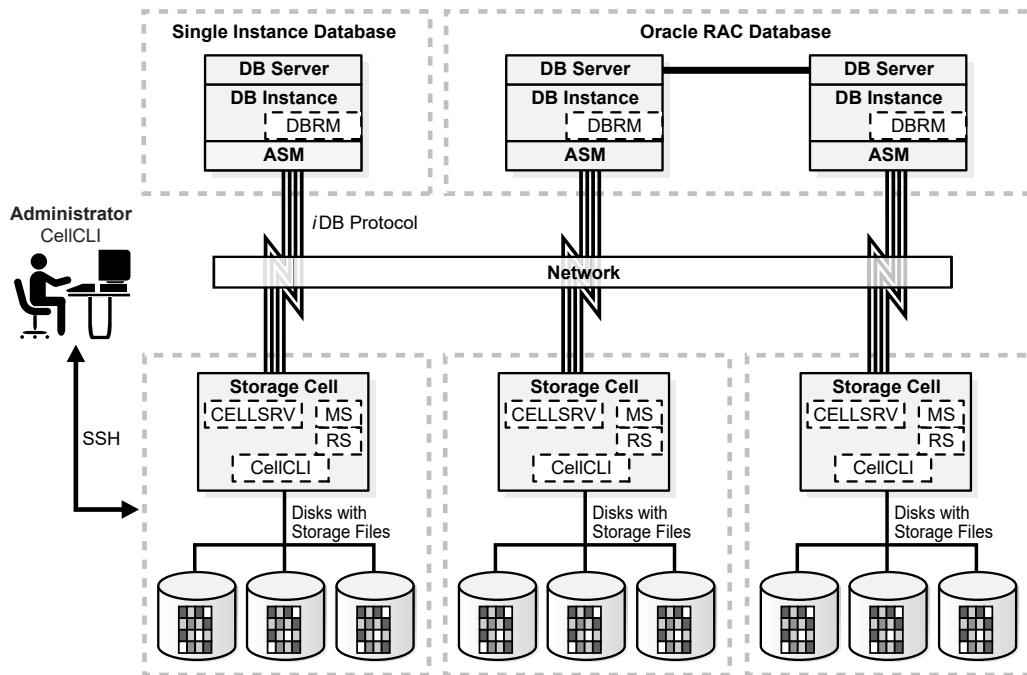
Figure 1-4 Software Components in the Exadata Database Machine Environment
