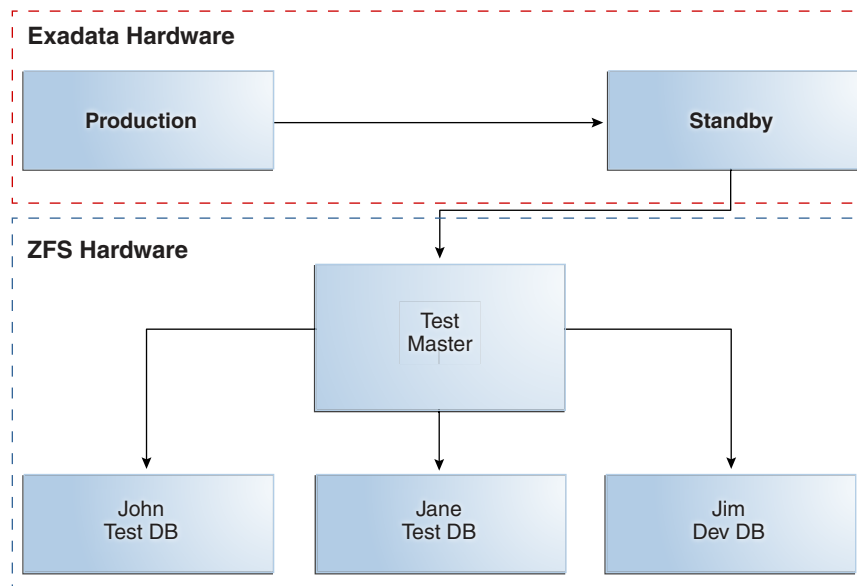
Figure 10-1 Traditional Clone to a Non-Exadata System
