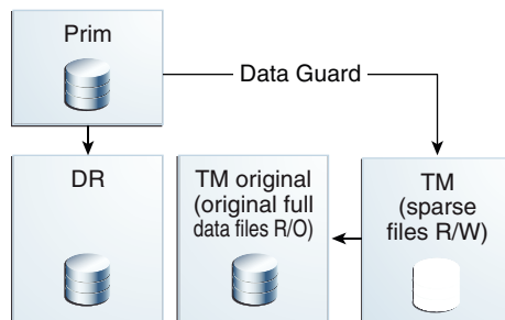
Figure 10-15 Configuration with Test Master Files and Sparse Files for Redo Apply
