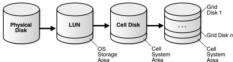
Figure 1-3 Oracle Exadata Storage Server Components
