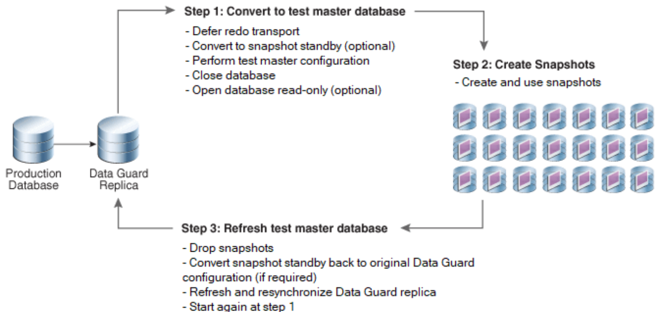
Figure 10-13 Lifecycle of Test Master and Snapshot Databases
