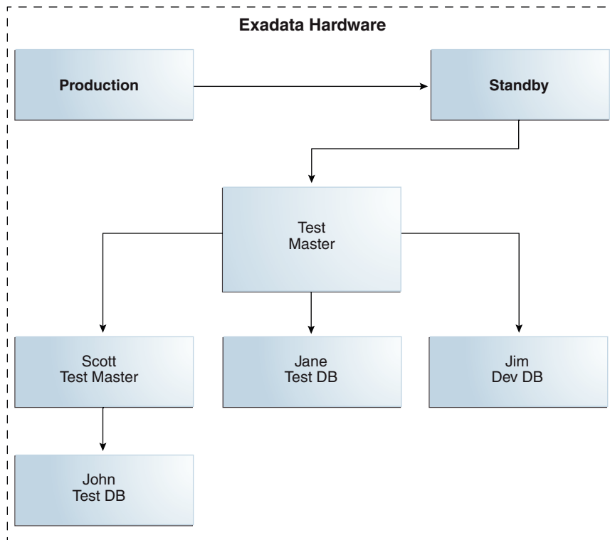
Figure 10-7 Hierarchical Snapshot Databases
