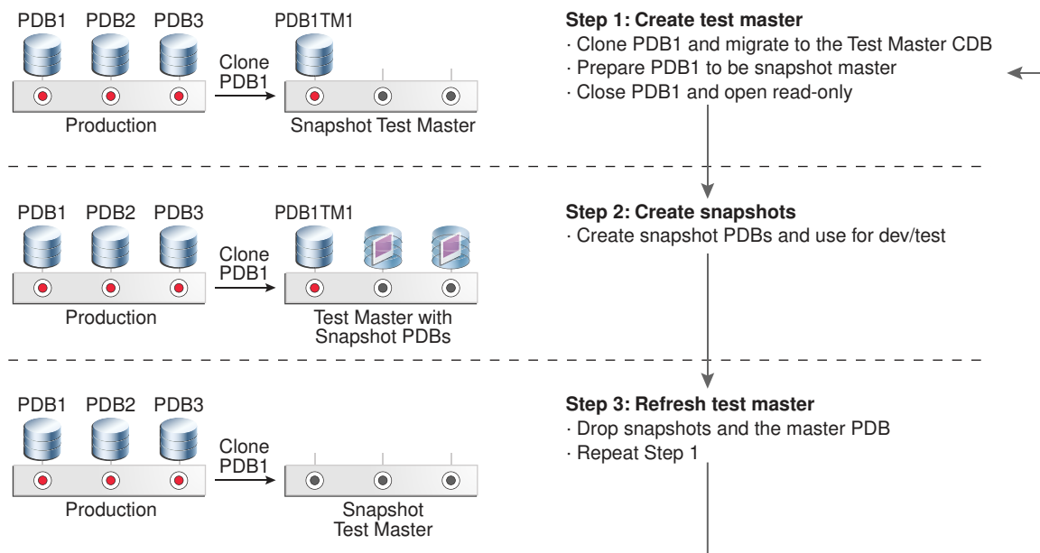
Figure 10-12 Lifecycle of Exadata Snapshots Using PDBs
