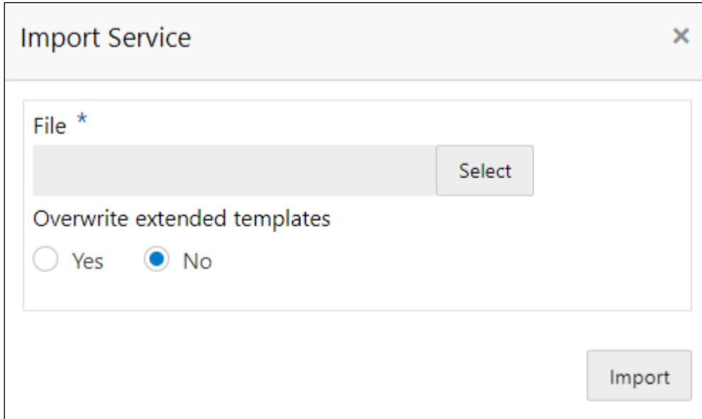
Figure 9: Import Service
