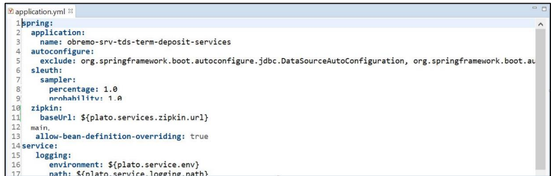
Figure 14: Application.yml File
