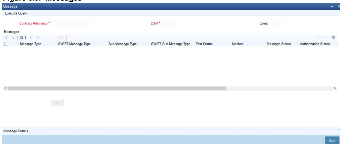
Figure 6.3: Messages
