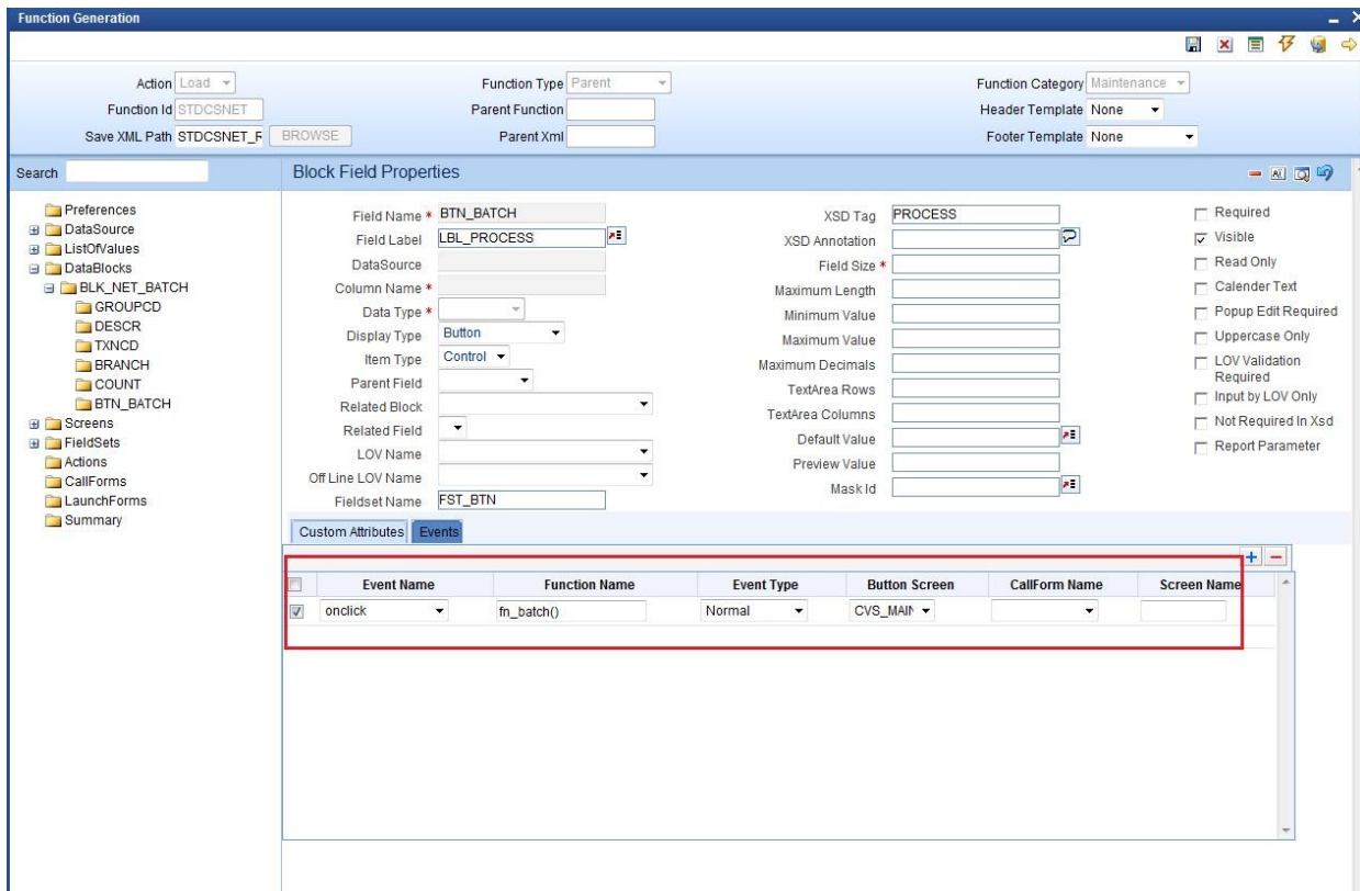
Fig 5.2 Button Field events : invoking a function on click of button
