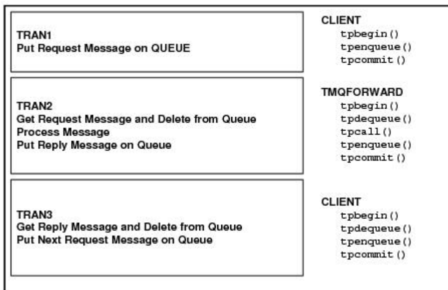
Figure 1-3 Transaction Demarcation
