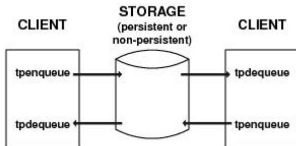
Figure 1-2 Peer-to-Peer Communication
