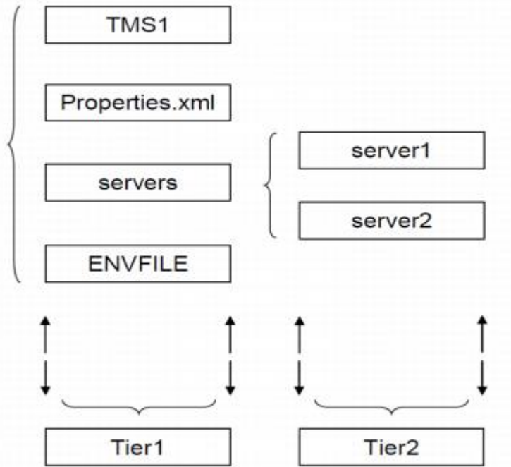
Figure 18-2 Application Package
