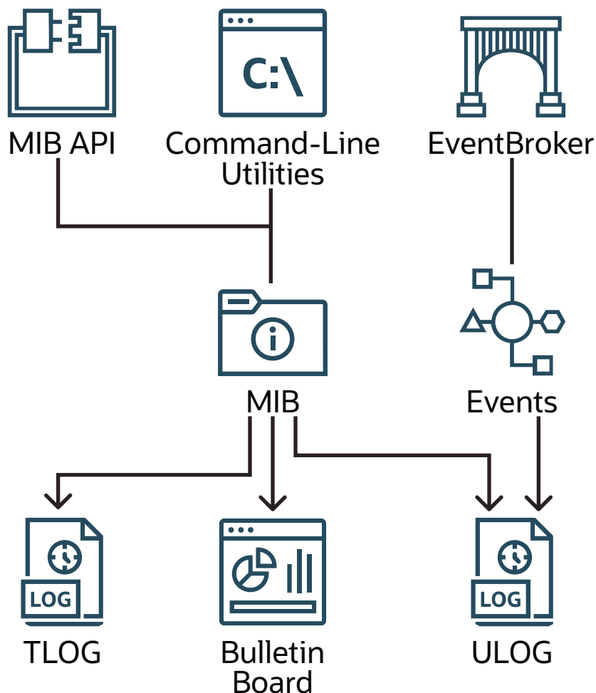
Figure 1-1 Administration Tools
