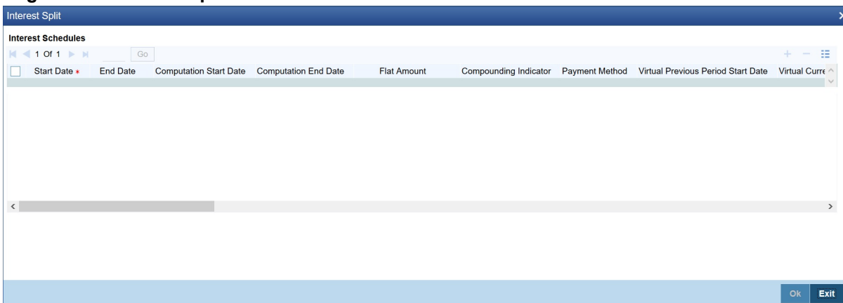
Figure 5.7: Interest Split
