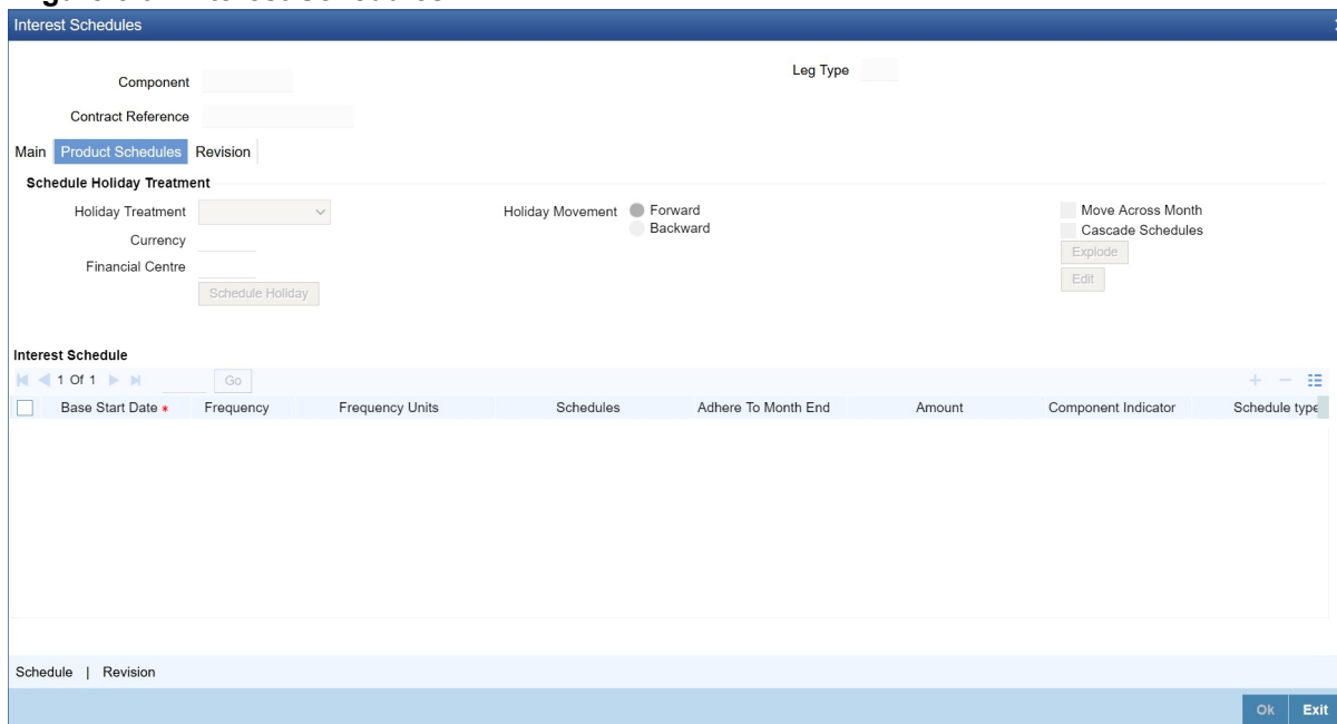
Figure 5.6: Interest Schedules
