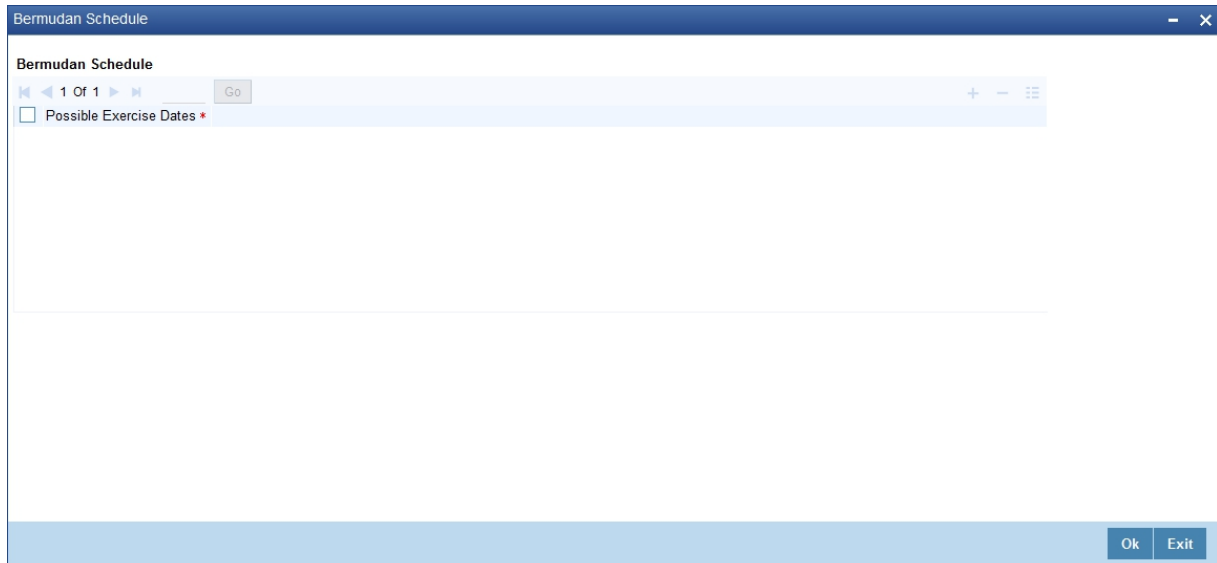
Figure 5.2: Bermudan Scheduler
