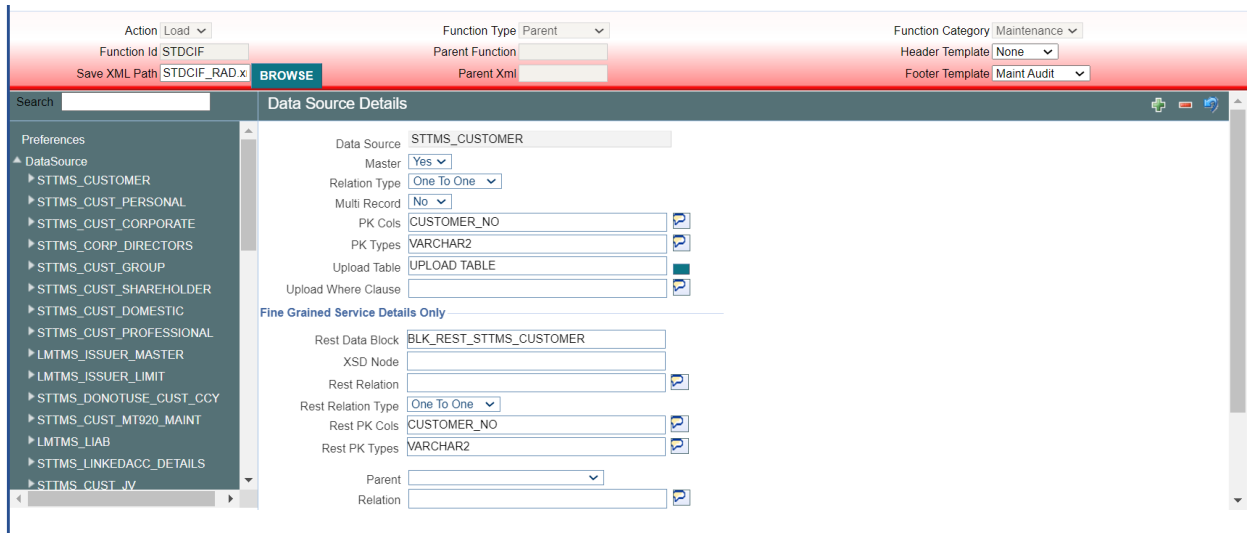
Fig 7.3 Data Source Properties
