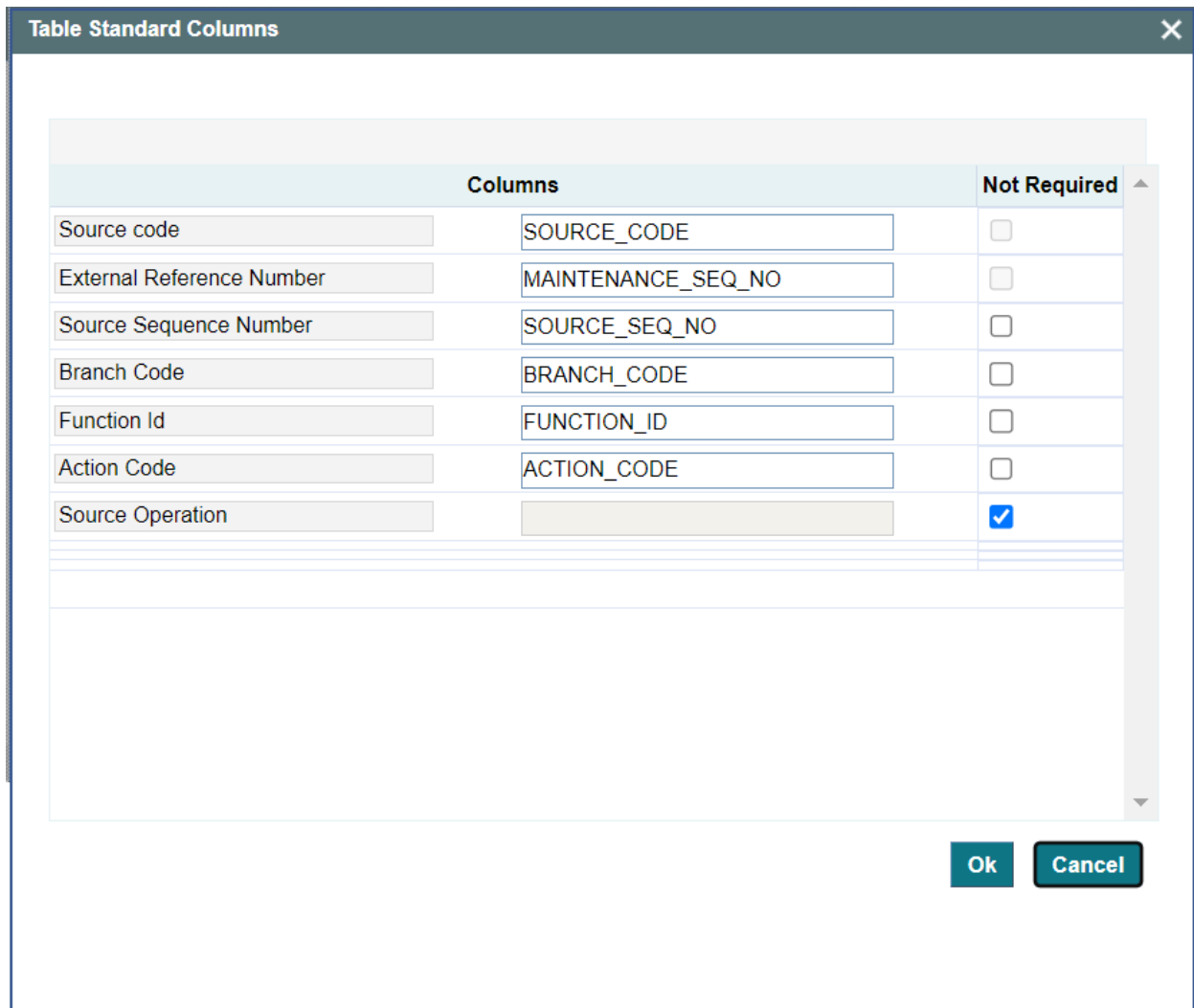
Fig 7.4 Adding Fields to created Data Source
