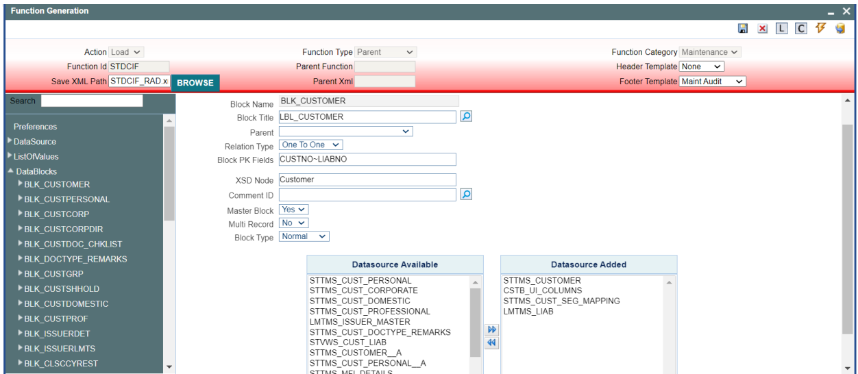
Fig 8.3 Data Block Properties
