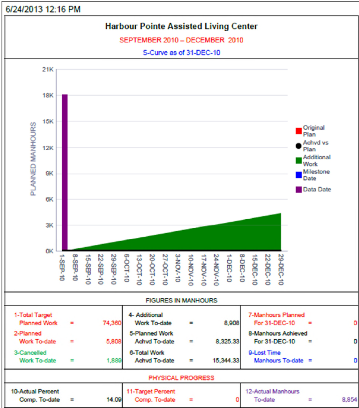
Figure 38: S Curve
