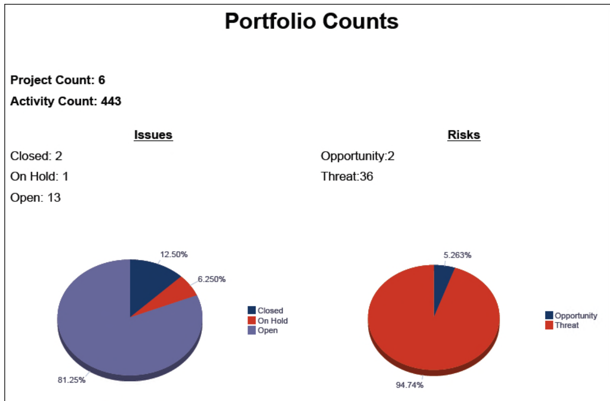
Figure 24: Portfolio Counts
