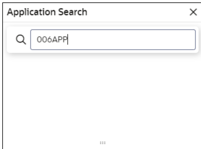
Figure 6: Application Search
