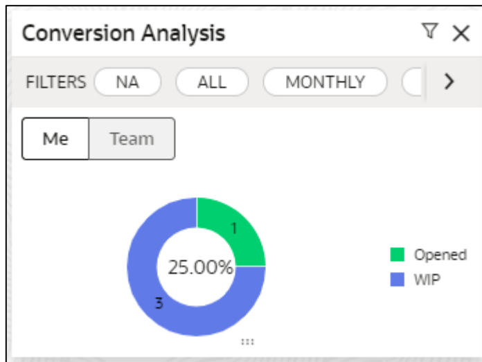
Figure 7: Conversion Analysis
