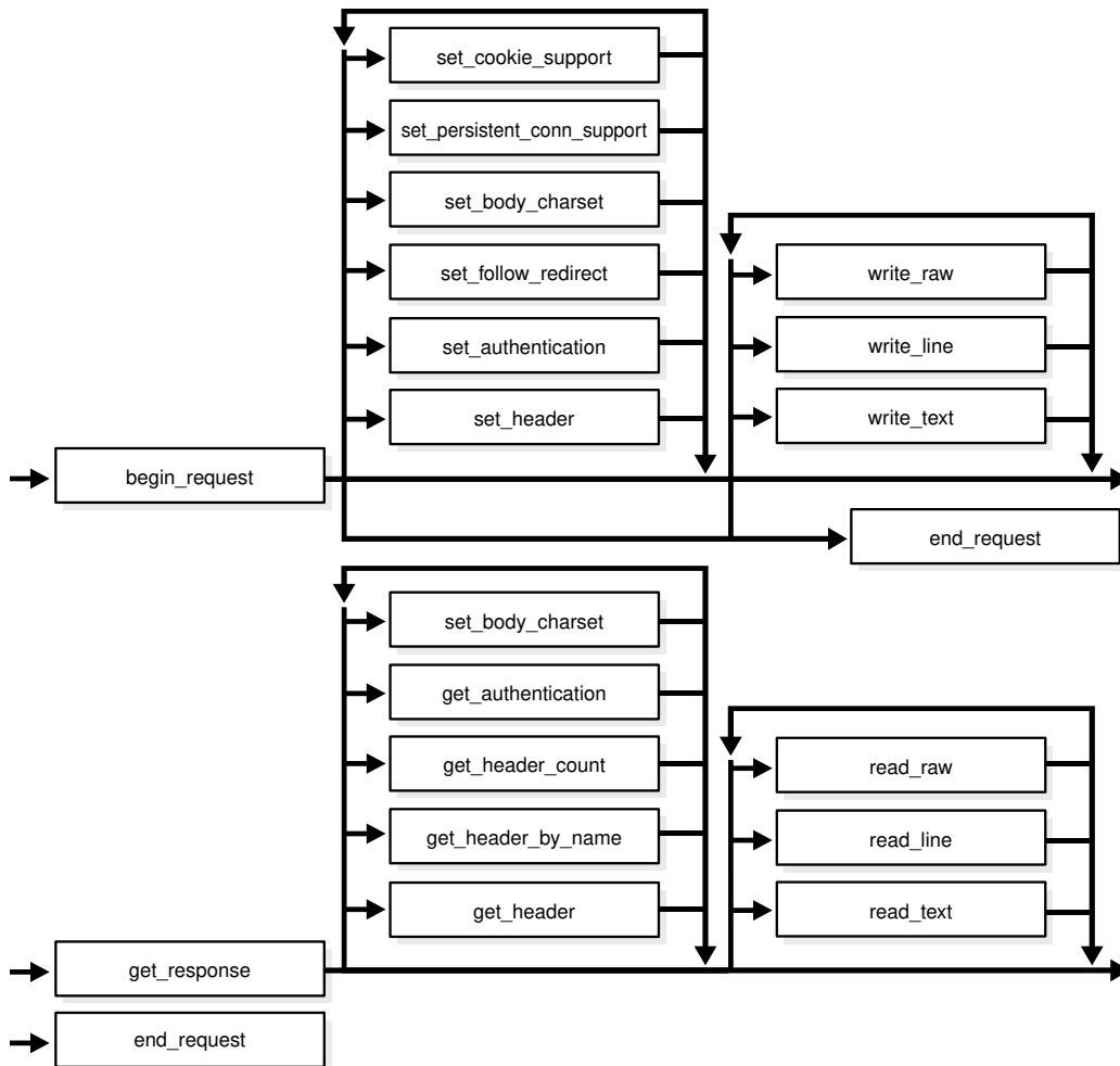
Figure 277-1 Flow of the Core UTL_HTTP Package
