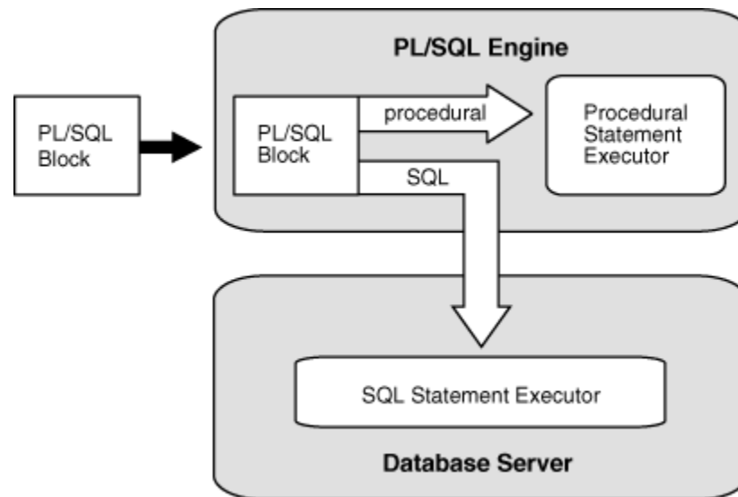
Figure 2-1 PL/SQL Engine
