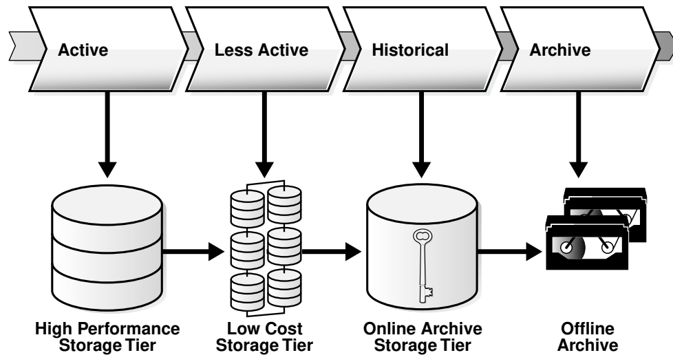
Figure 5-3 Data Lifecycle
