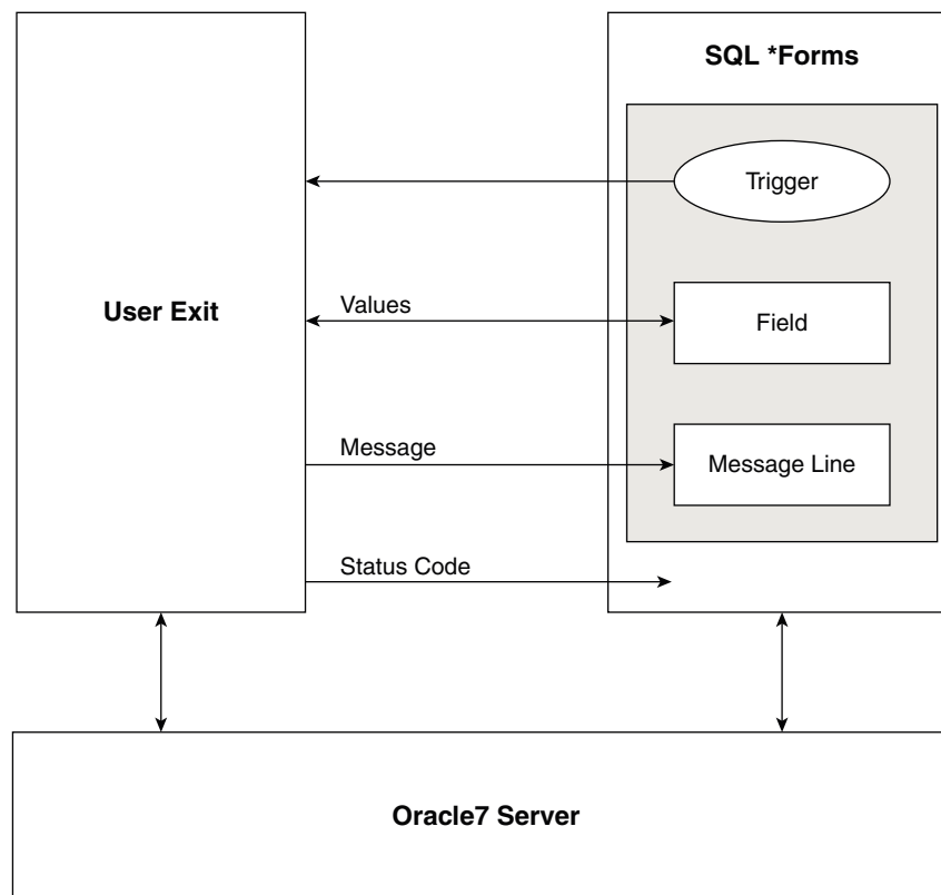
Figure 11-1 SQL*Forms
