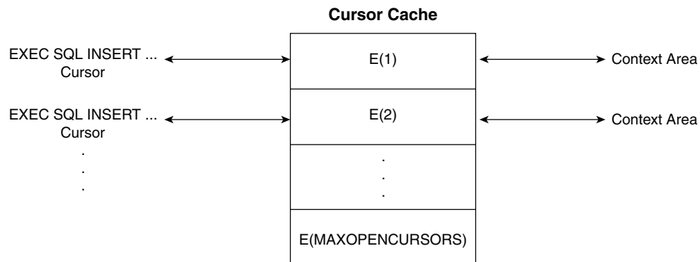
Figure C-2 Cursors Linked through the Cursor Cache
