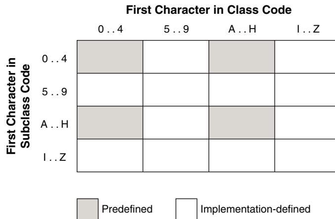
Figure 8-1 SQLSTATE Coding Scheme
