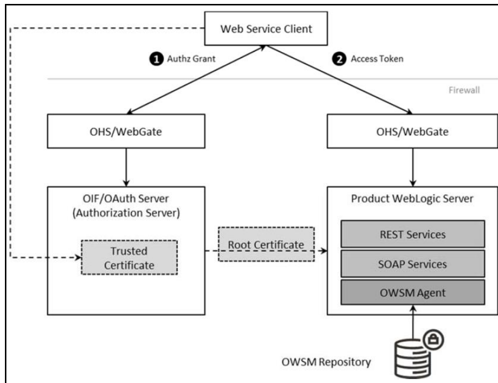
Figure 9: Federated Web Services Process Flow
