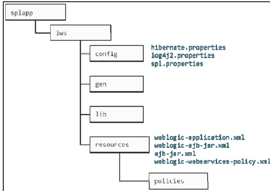
Figure 26: Inbound Web Services Structures
