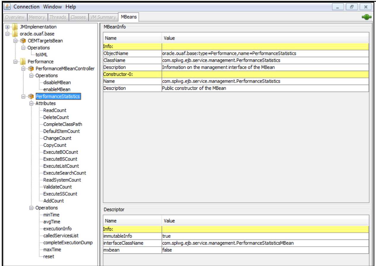
Figure 11: Business Application Server Mbeans in jconsole Example
