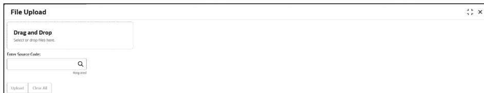
Figure 7: File Upload
