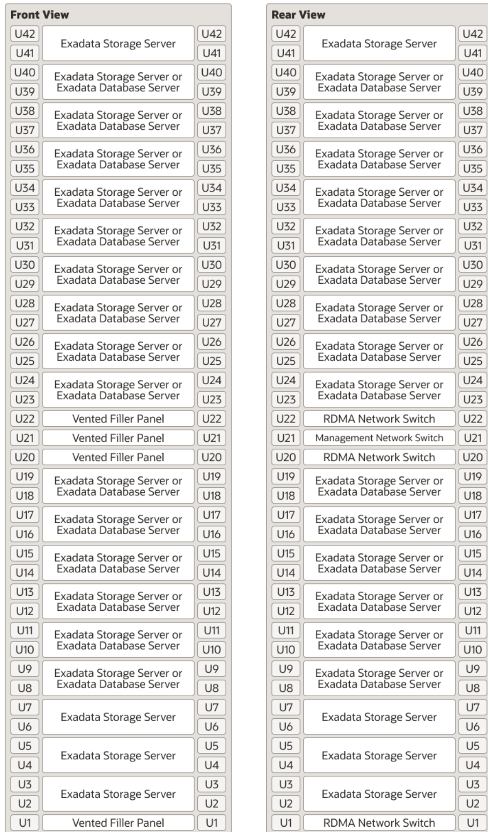
Figure 12-1 Rack Layout for Oracle Exadata Database Machine X10M
