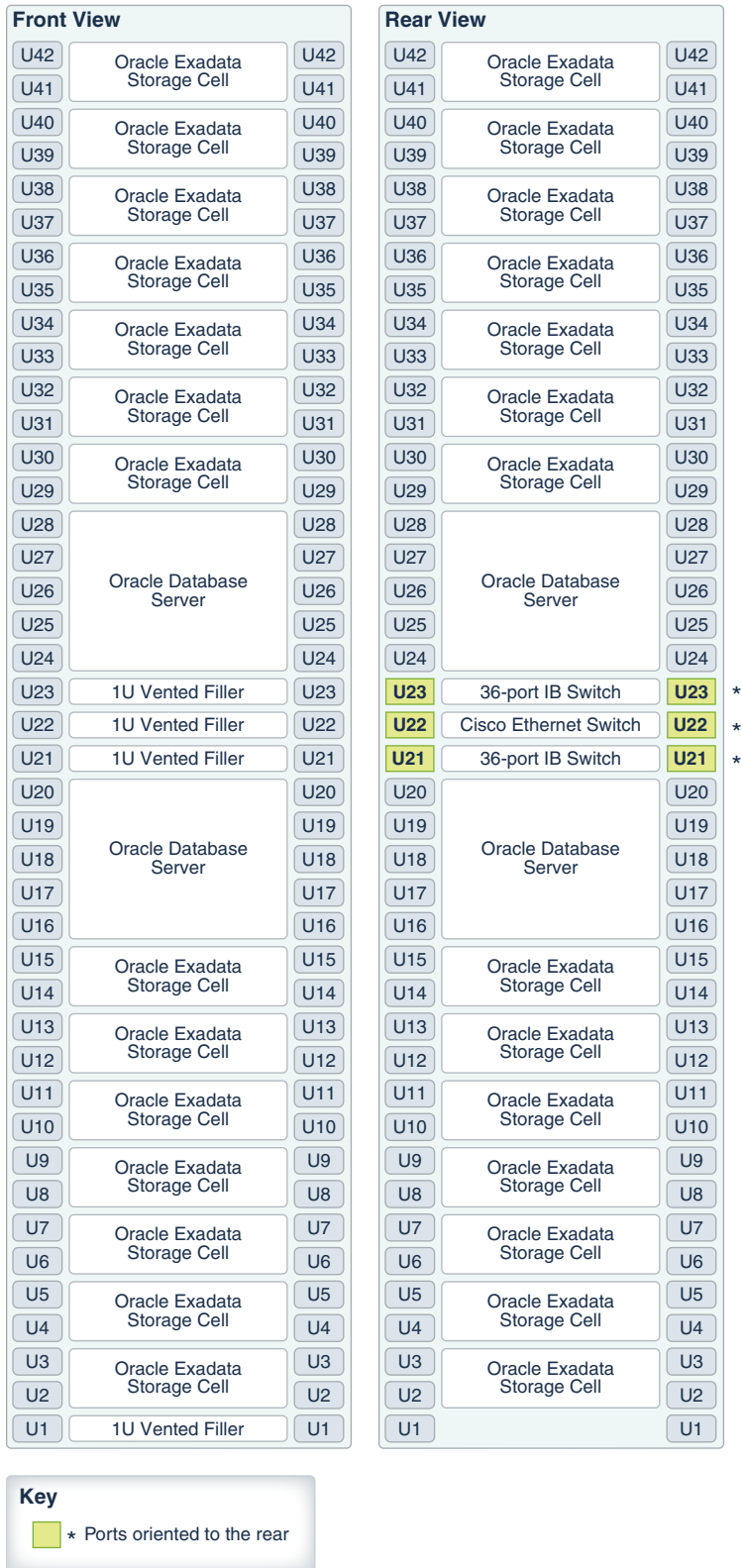
Figure 15-2 Rack Layout of Oracle Exadata Database Machine X8-8 and X7-8
