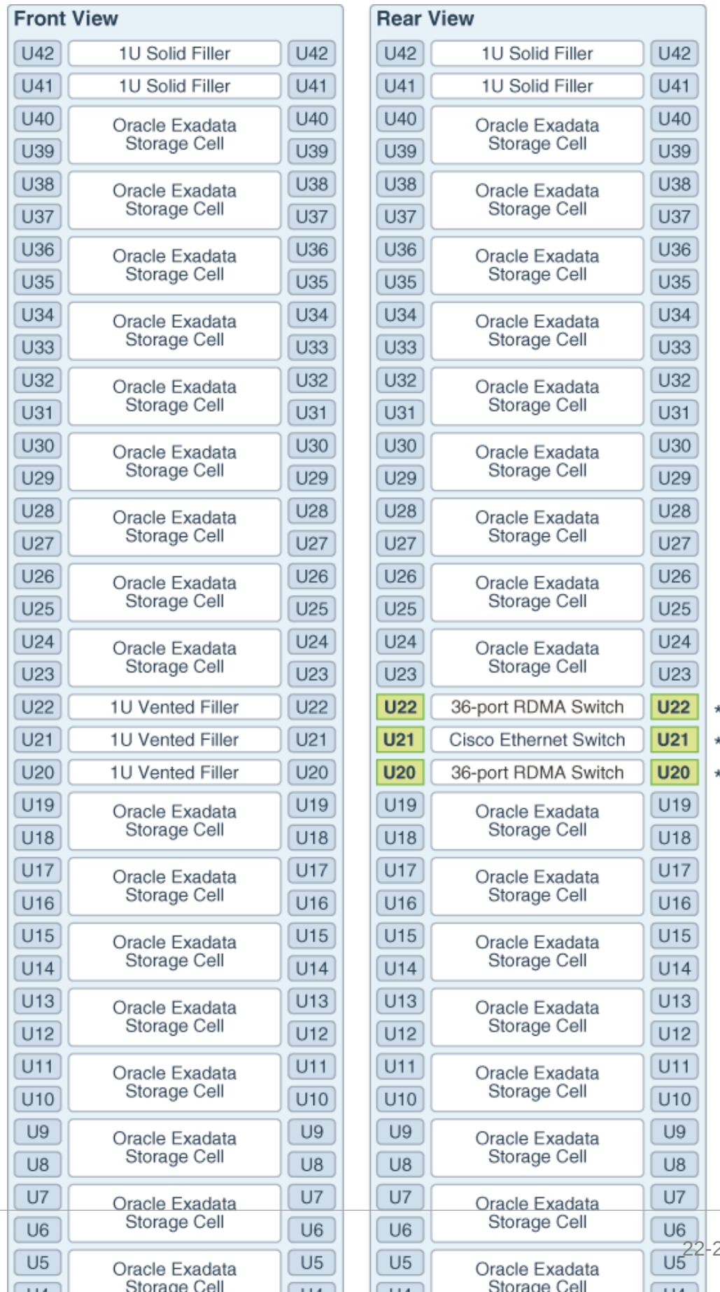
Figure 22-1 Rack Layout of Oracle Exadata Storage Expansion Full Rack X5 to X8M
