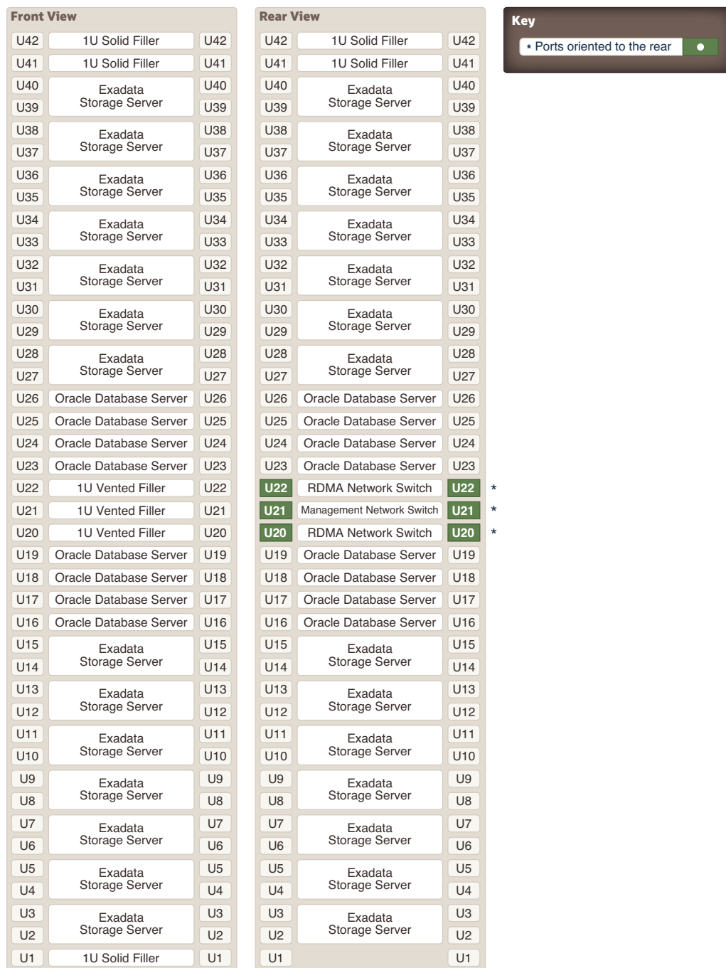
Figure 14-1 Rack Layout of Oracle Exadata X8M-2 Full Rack
