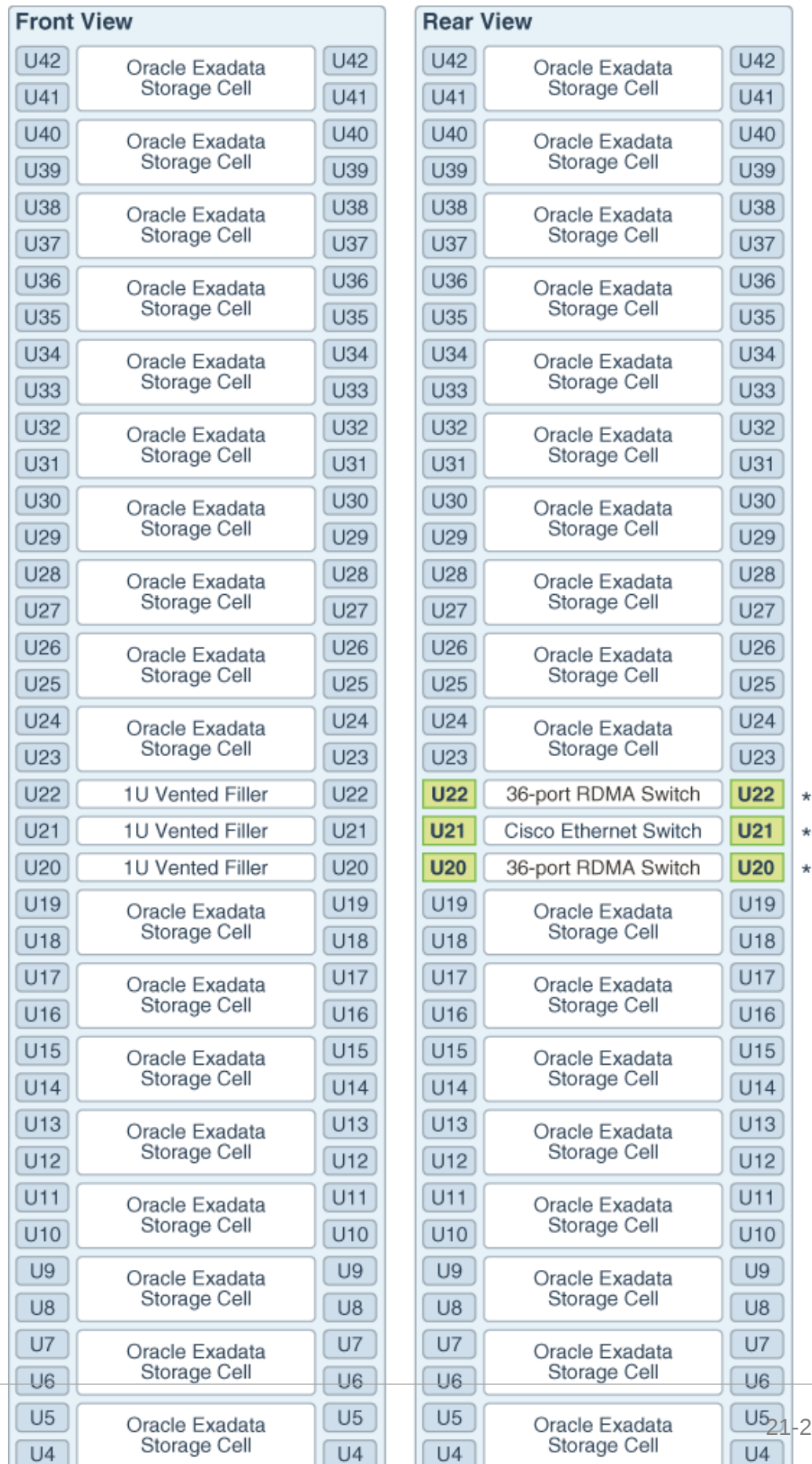
Figure 21-1 Rack Layout of Oracle Exadata Storage Expansion Rack X9M-2
