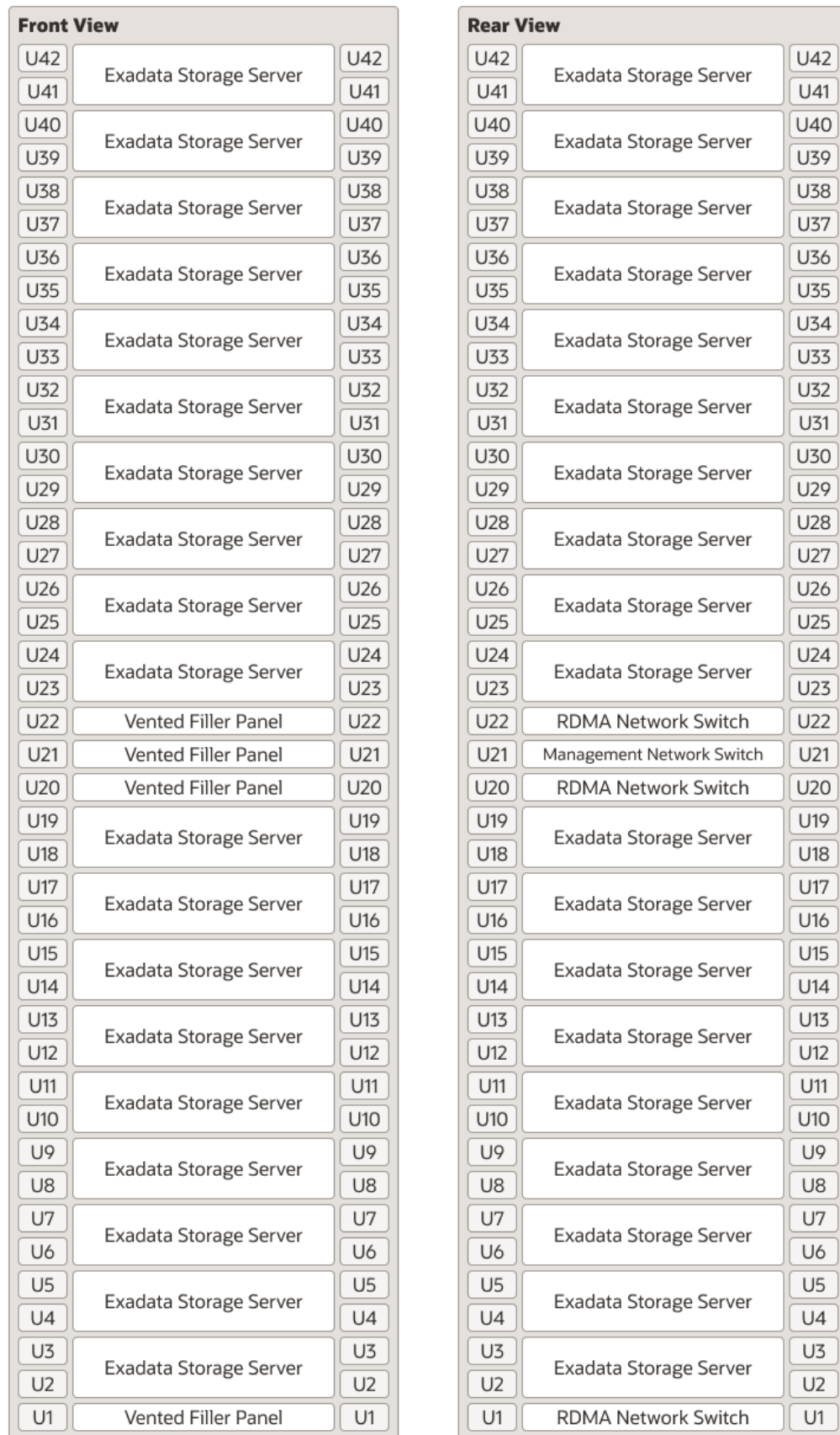
Figure 20-1 Rack Layout for Oracle Exadata Storage Expansion Rack X10M
