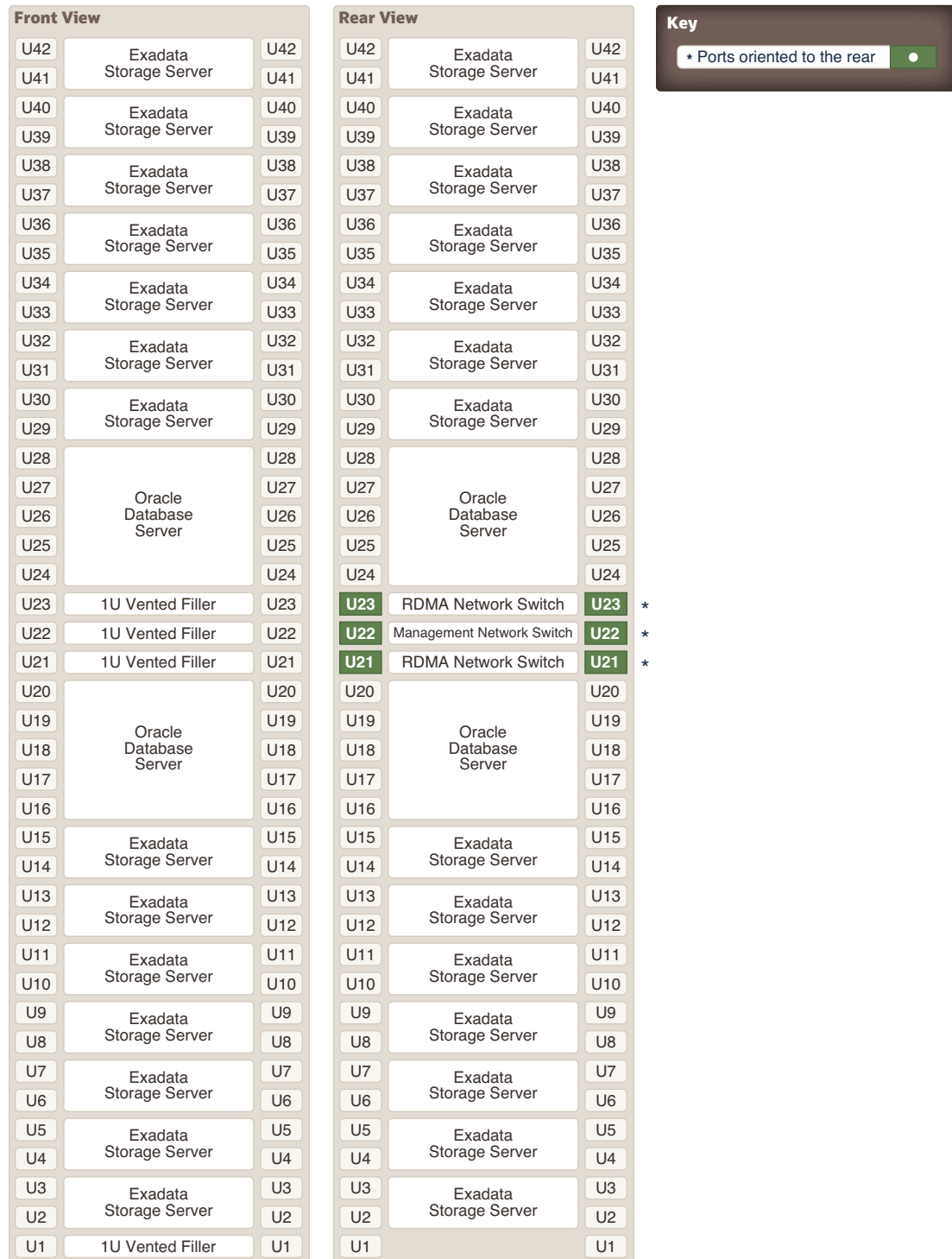
Figure 14-2 Rack Layout of Oracle Exadata X8M-8
