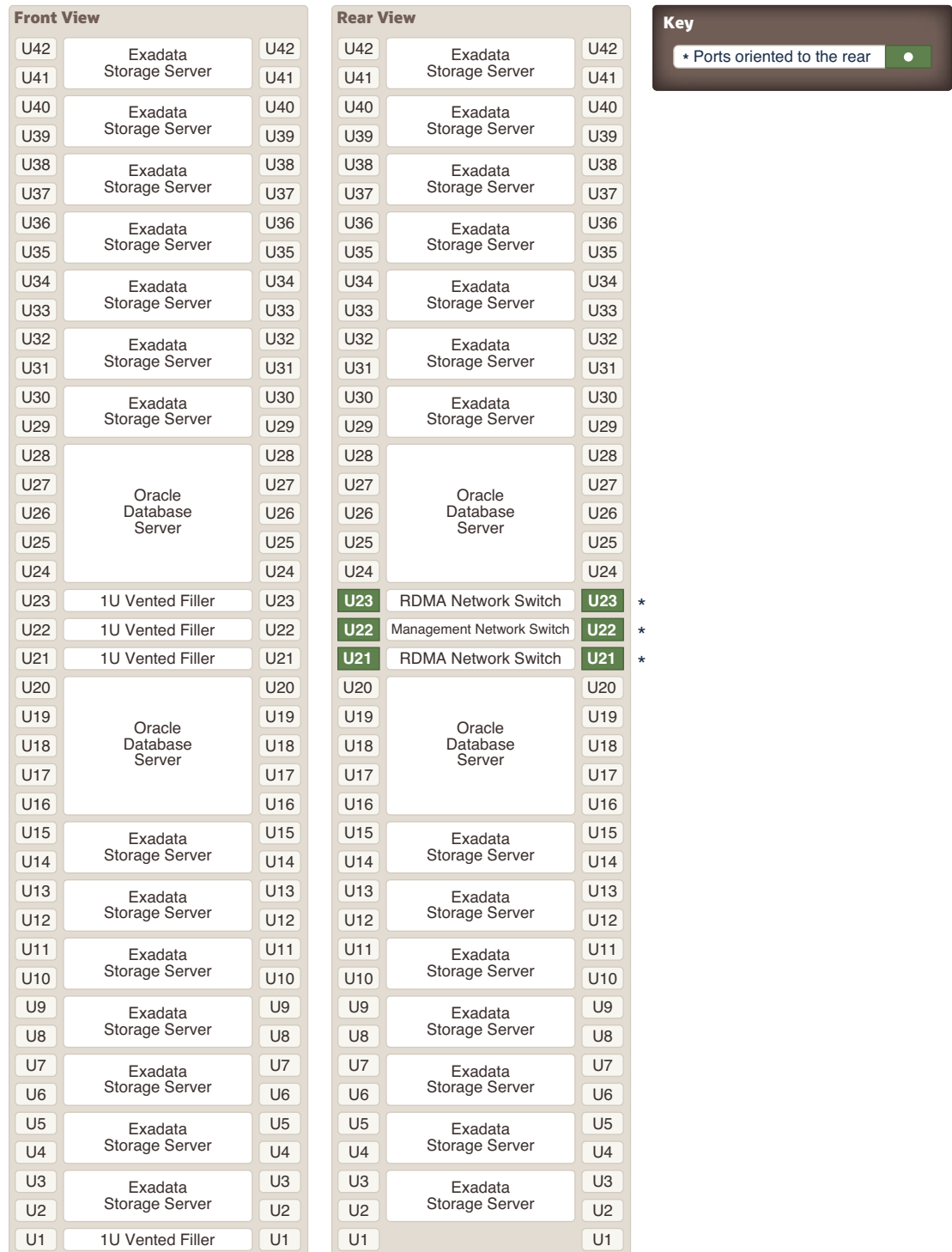
Figure 13-2 Rack Layout of Oracle Exadata X9M-8
