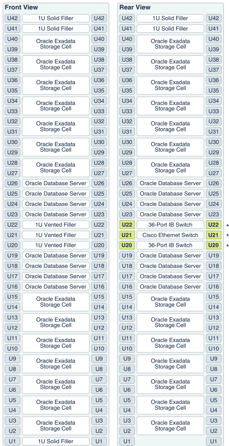
Figure 15-1 Rack Layout of Oracle Exadata Database Machine X8-2 and X7-2 Full Rack
