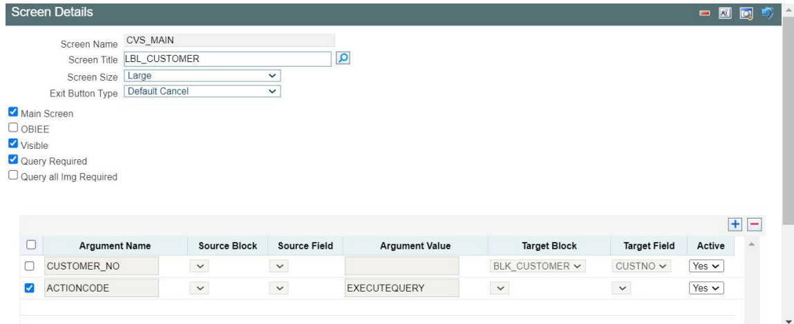
Fig 9.3 Screen Properties
