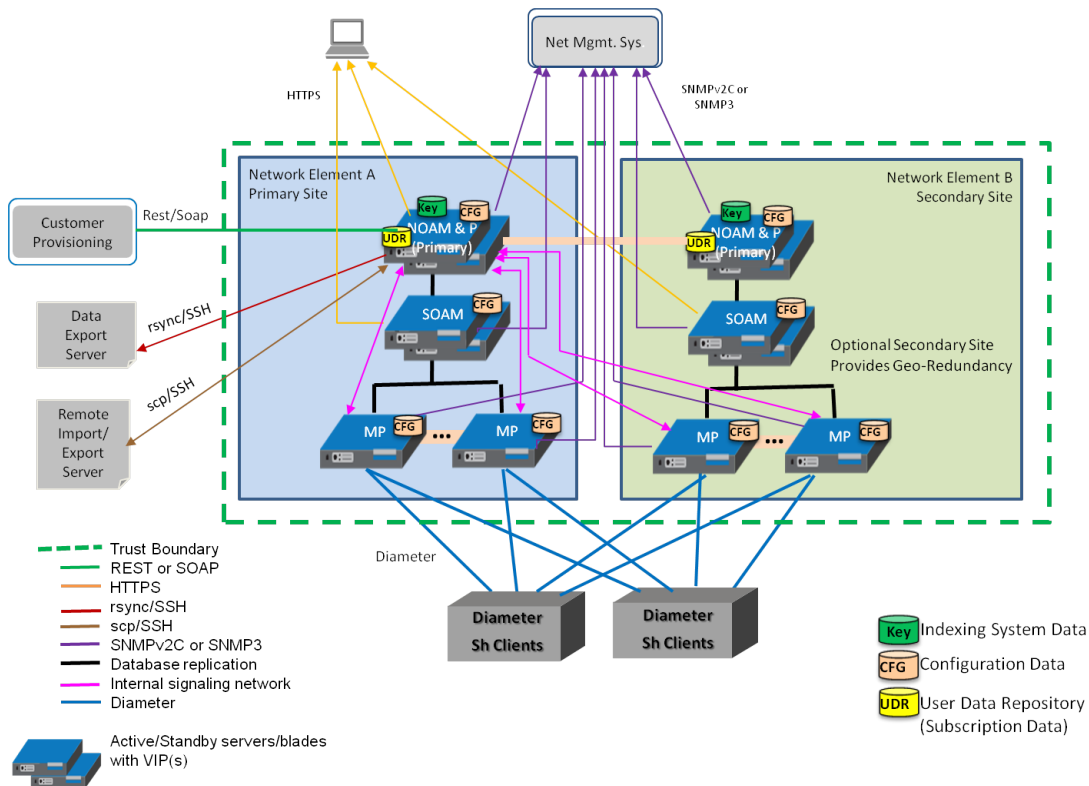
Figure 3-1 UDR System Architecture
