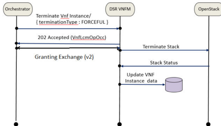
Figure 14-1 Forceful termination
