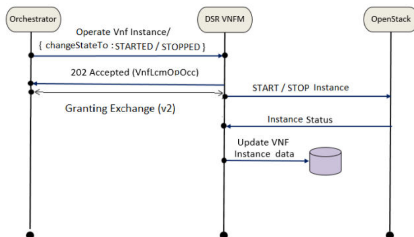
Figure 9-8 Operate vnf
