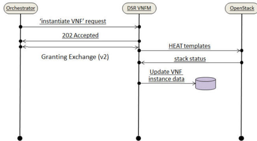
Figure 9-5 VNF installation
