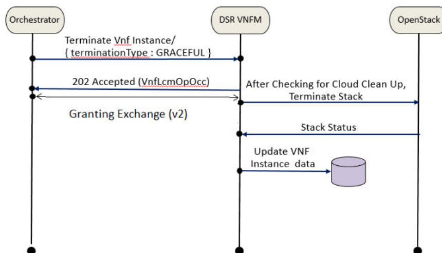
Figure 14-2 Graceful termination
