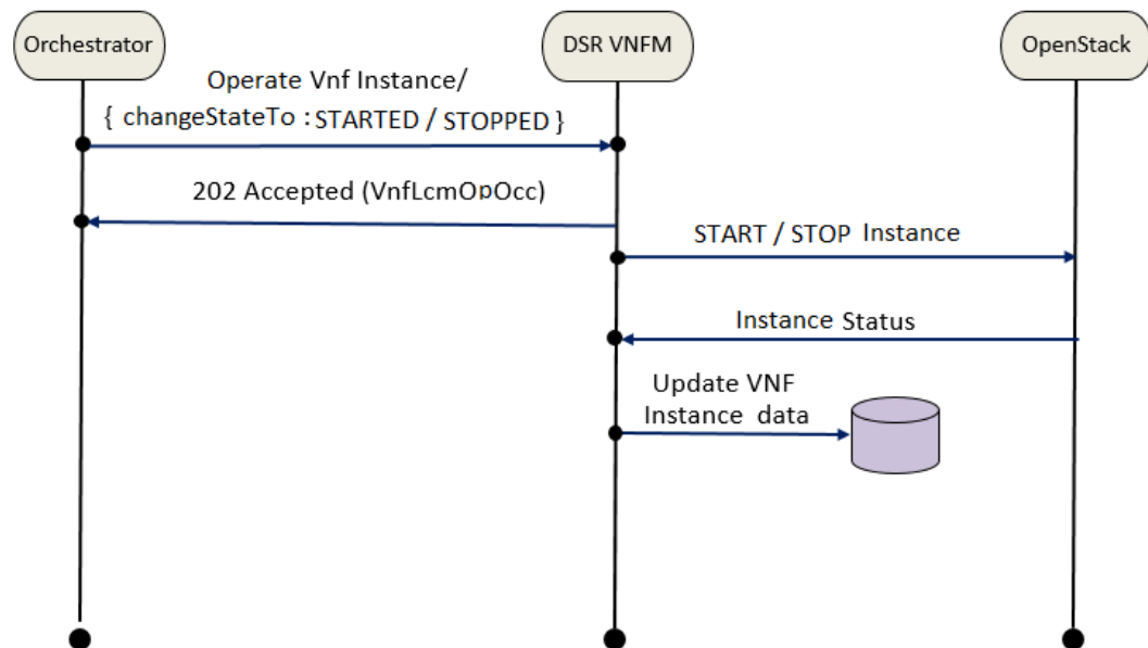
Figure 9-8 Operate VNF
