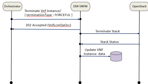
Figure 14-1 Forceful Termination
