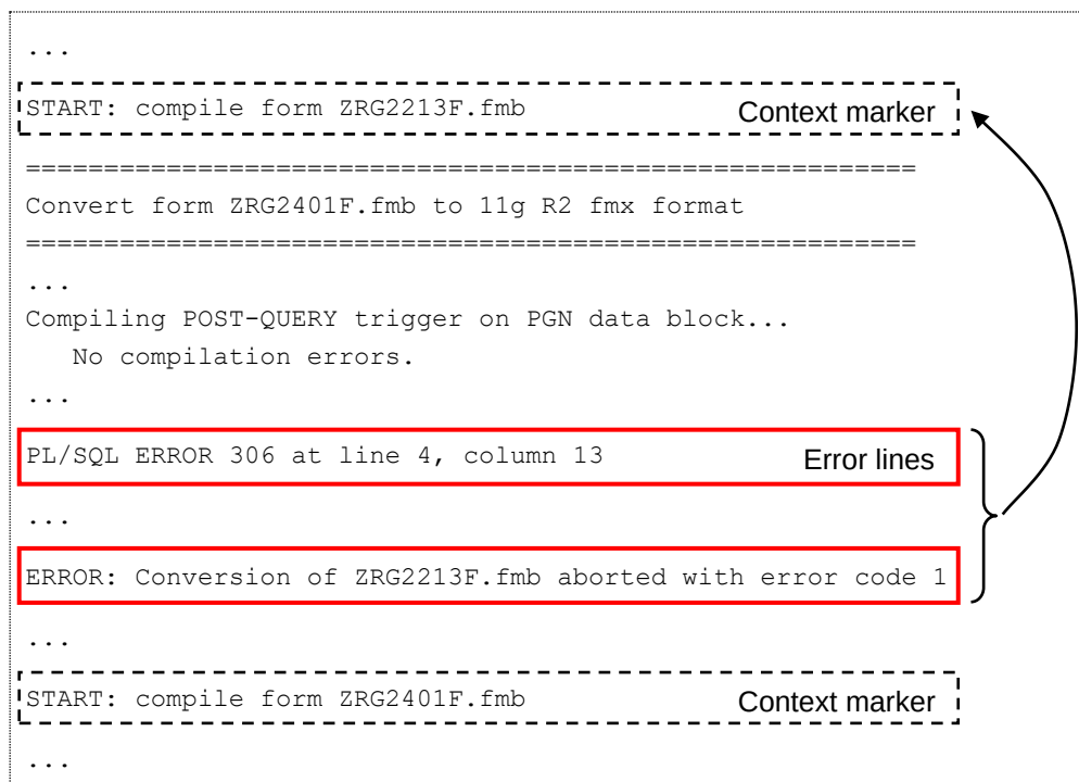
Figure 2: error lines in an activity's log file are captured by context
