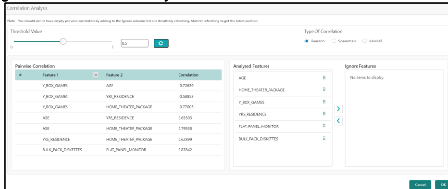
Figure 259: Correlation Analysis - Pairwise Correlation
