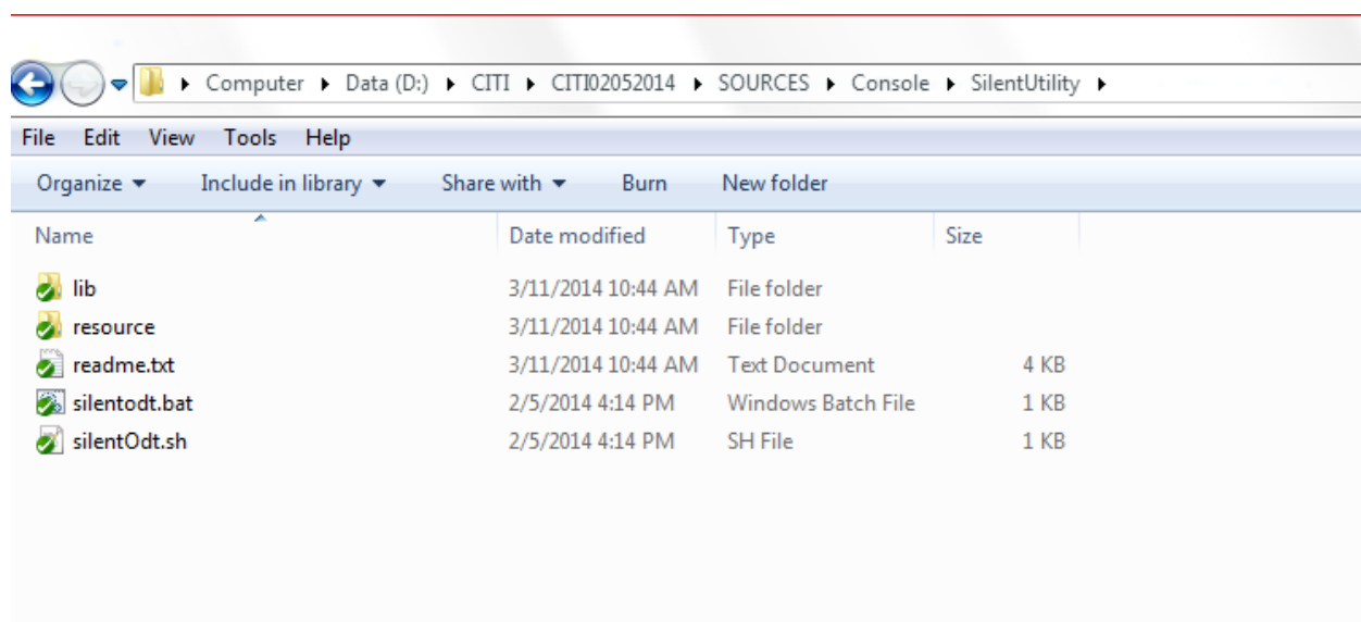
Fig 4.4.1: SilentODT Sources
