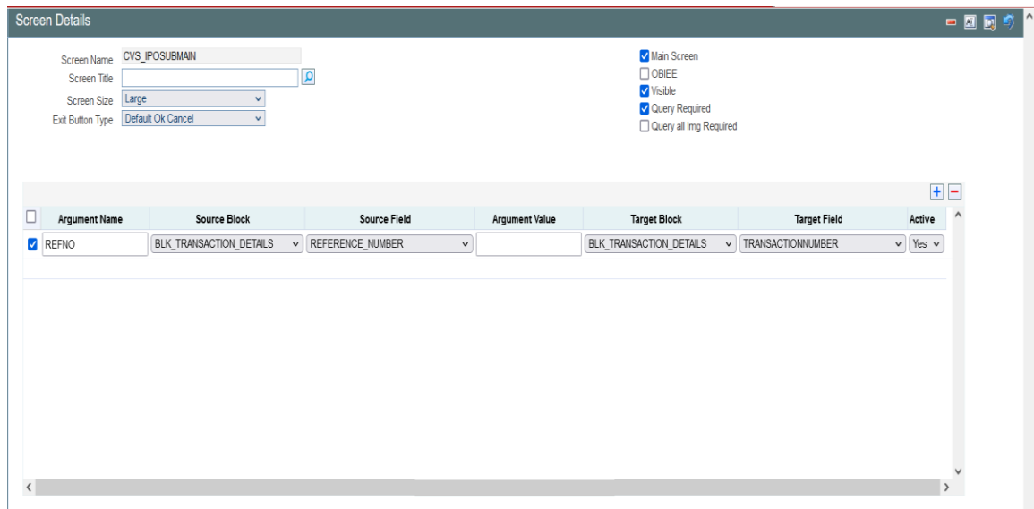
Fig: Defining Screen arguments for a Screen
