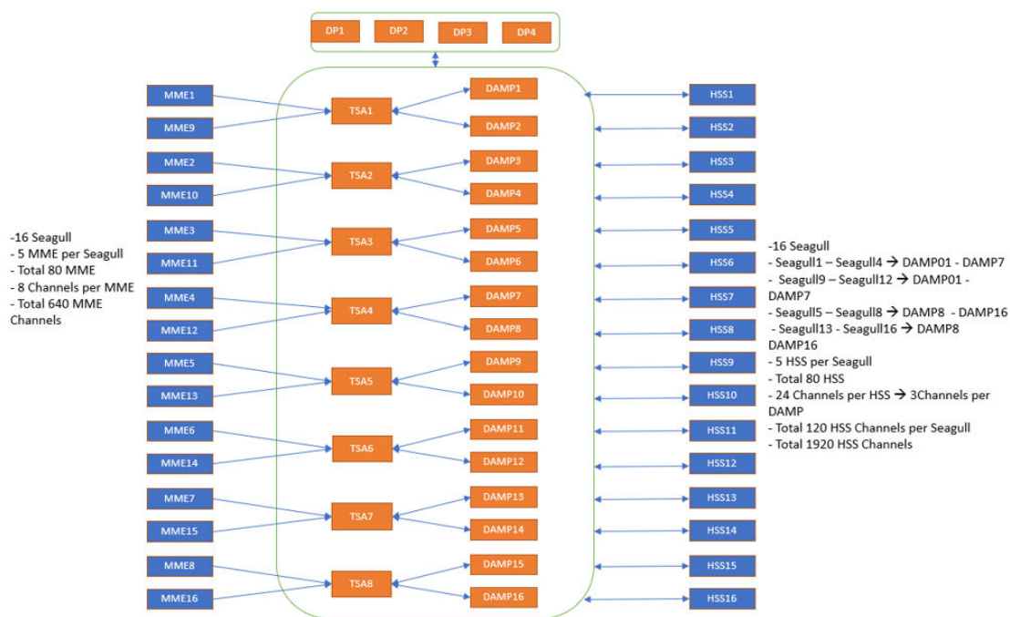
Figure F-1 Topology for KVM/Oracle X9-2 server with 24 vCPU Profile
