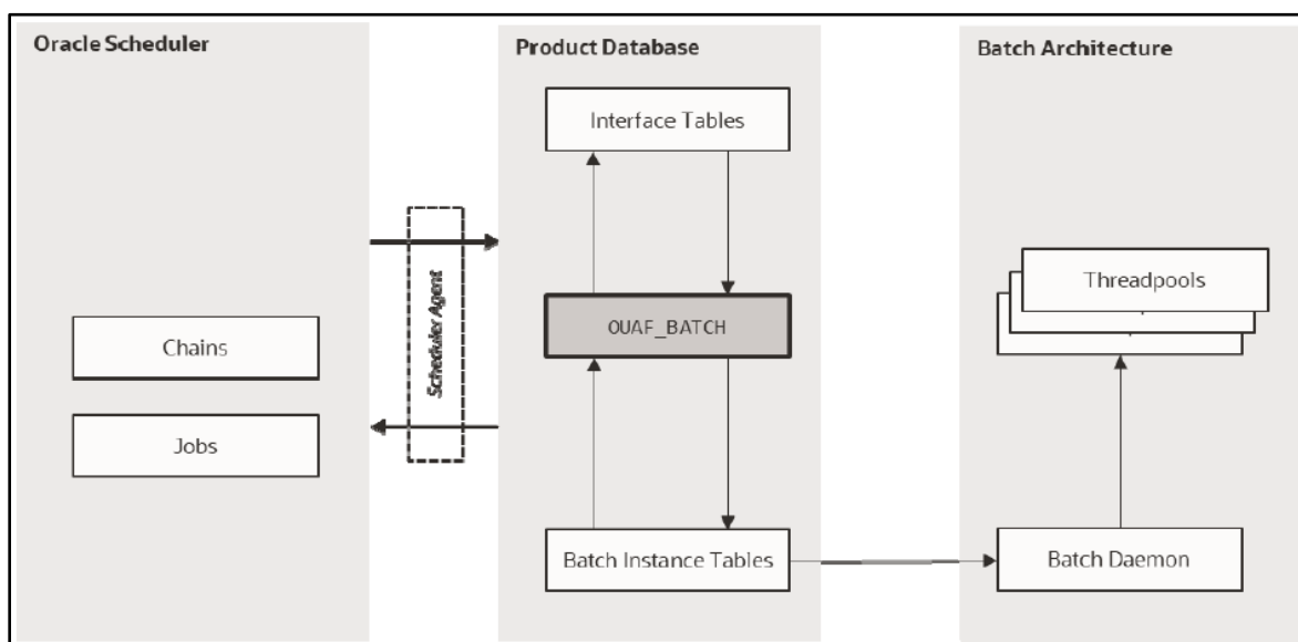
Figure 45: Oracle Scheduler Interface
