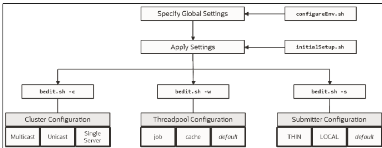
Figure 32: bedit Configuration Process
