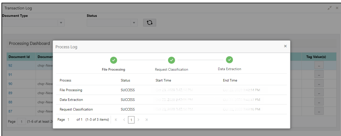
Figure 251: Execution Flow
