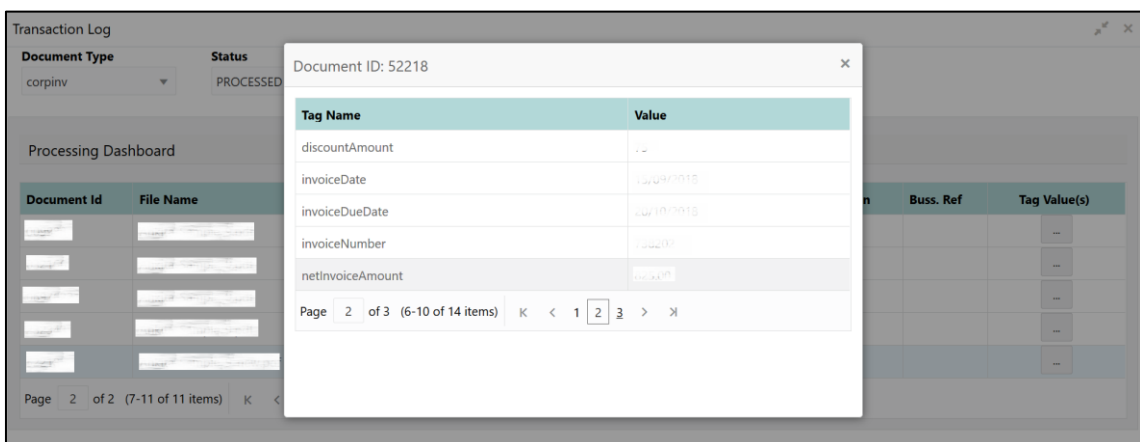
Figure 252: Processed Status
