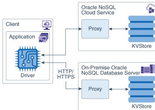
Figure 3-1 Oracle NoSQL Database Proxy and Driver
