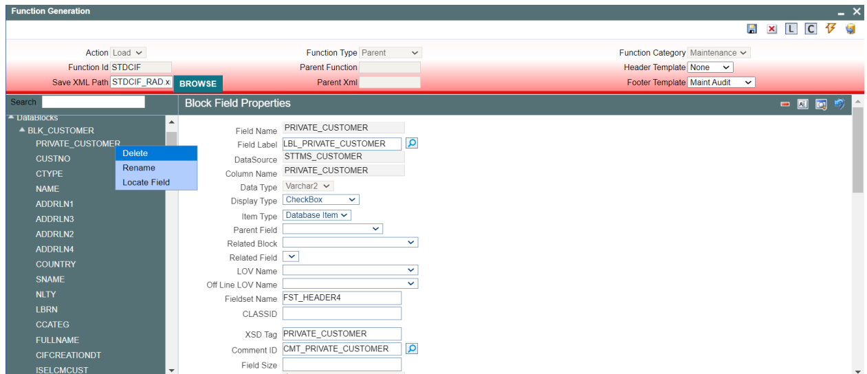
Fig 8.20 Deleting a Data Block Field
