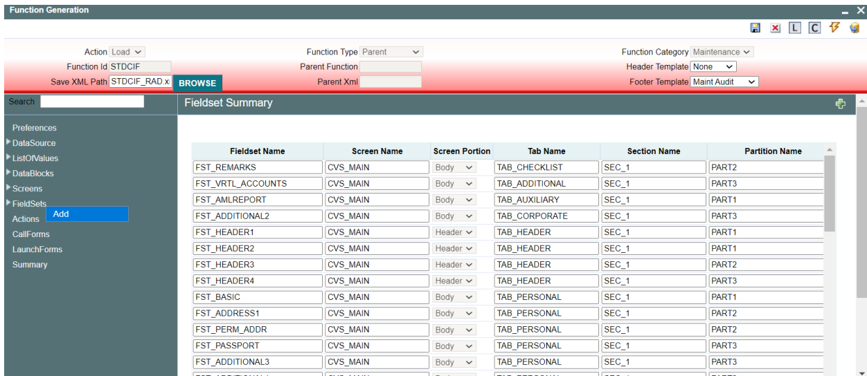
Fig 10.1 Adding a New Field Set
