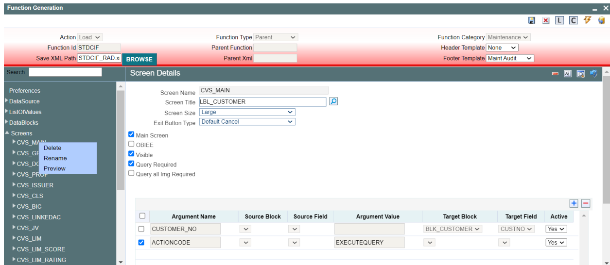
Fig 9.16 Renaming of Screen
