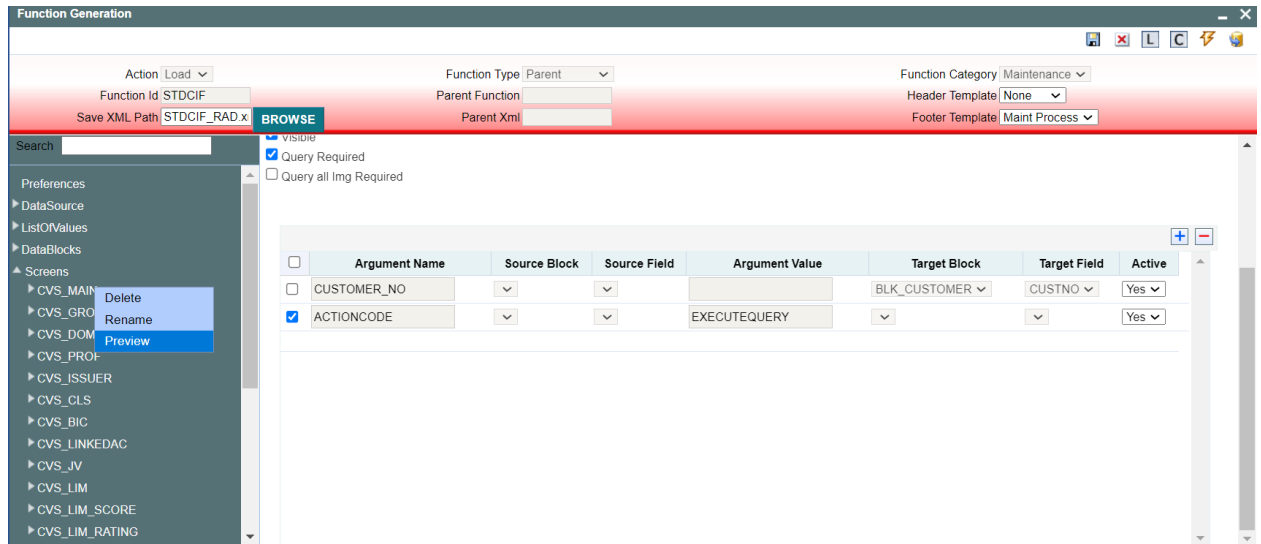
Fig 17.1 Previewing a Screen
