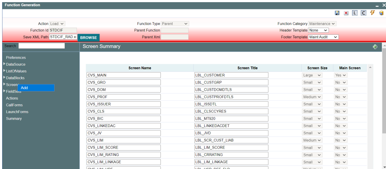
Fig 9.1 Adding a New Screen
