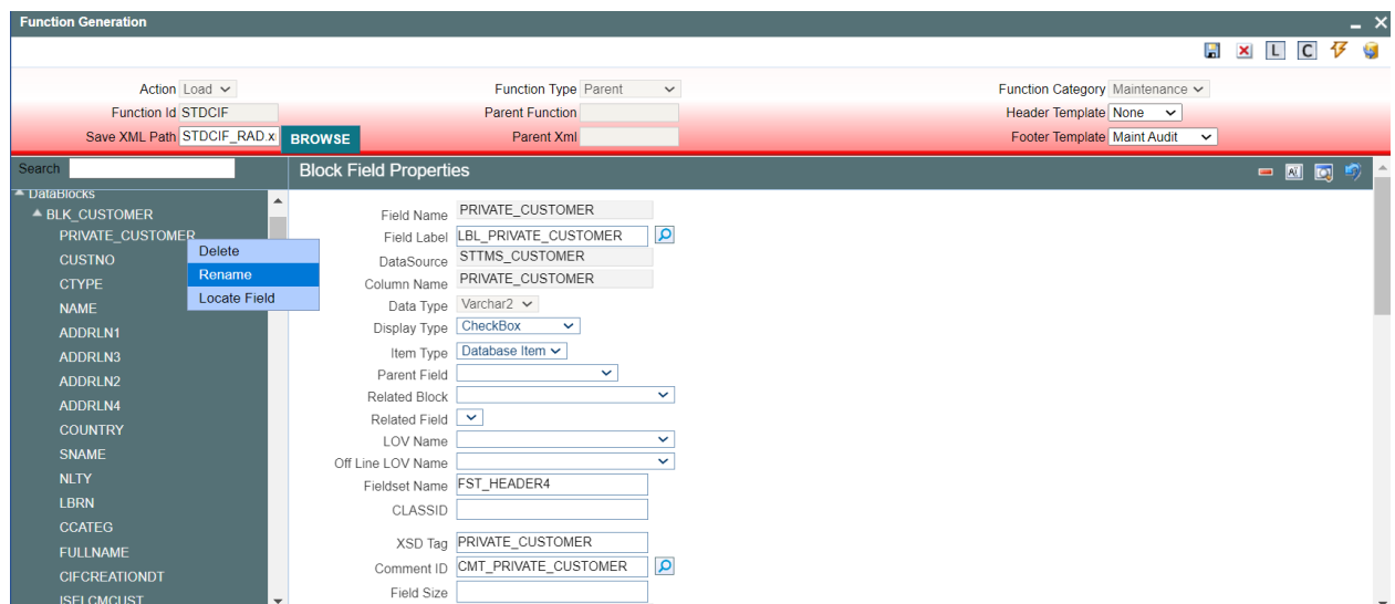
Fig 8.21 Renaming a Data Block
