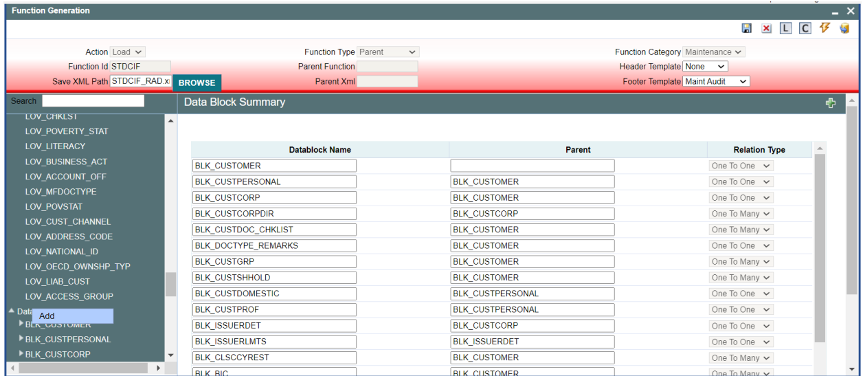
Fig 8.1 Adding a New Data Block
