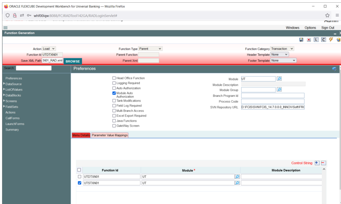
Fig: Preferences Screen highlighting SVN Repository URL
