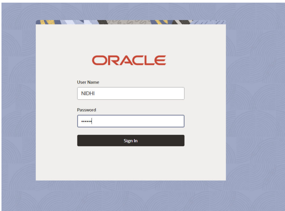
Figure 2-1 Login Screen
