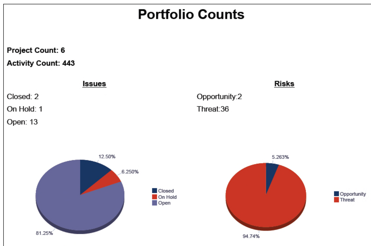
Figure 35: Portfolio Counts
