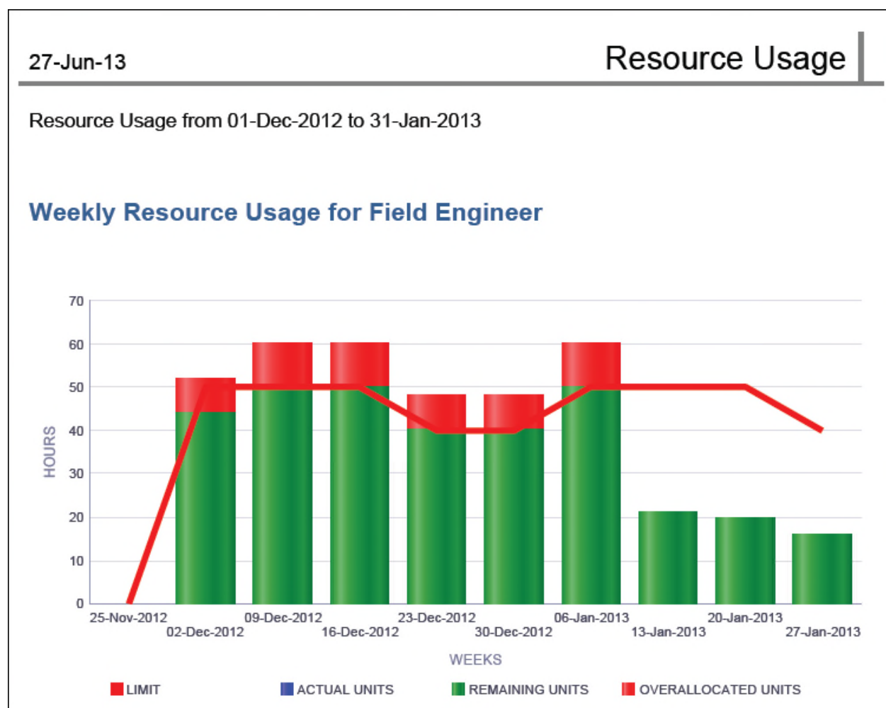
Figure 48: Limit Line
