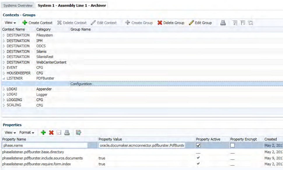
Figure 15: PDFBursting
