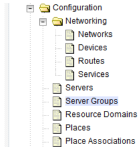
Figure 13-4 Server Groups
