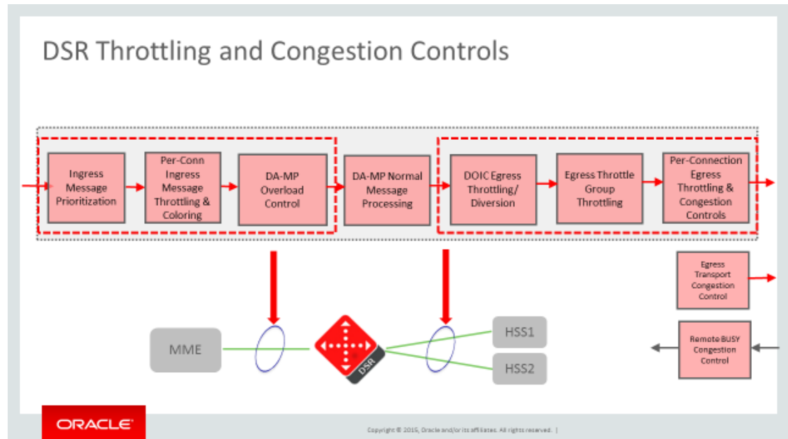
Figure 2-17 Congestion Control
