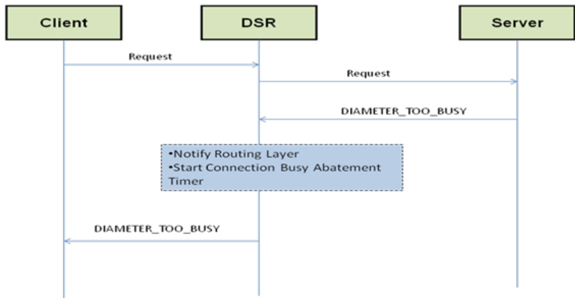
Figure 2-24 Connection Busy
