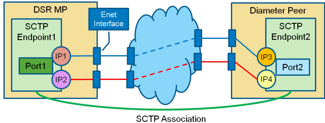
Figure 2-11 SCTP Multi-Homing
