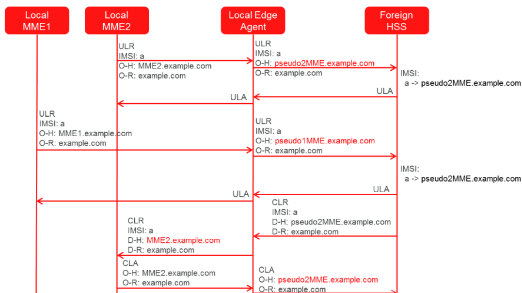
Figure 2-45 MME/SGSN Topology Hiding
