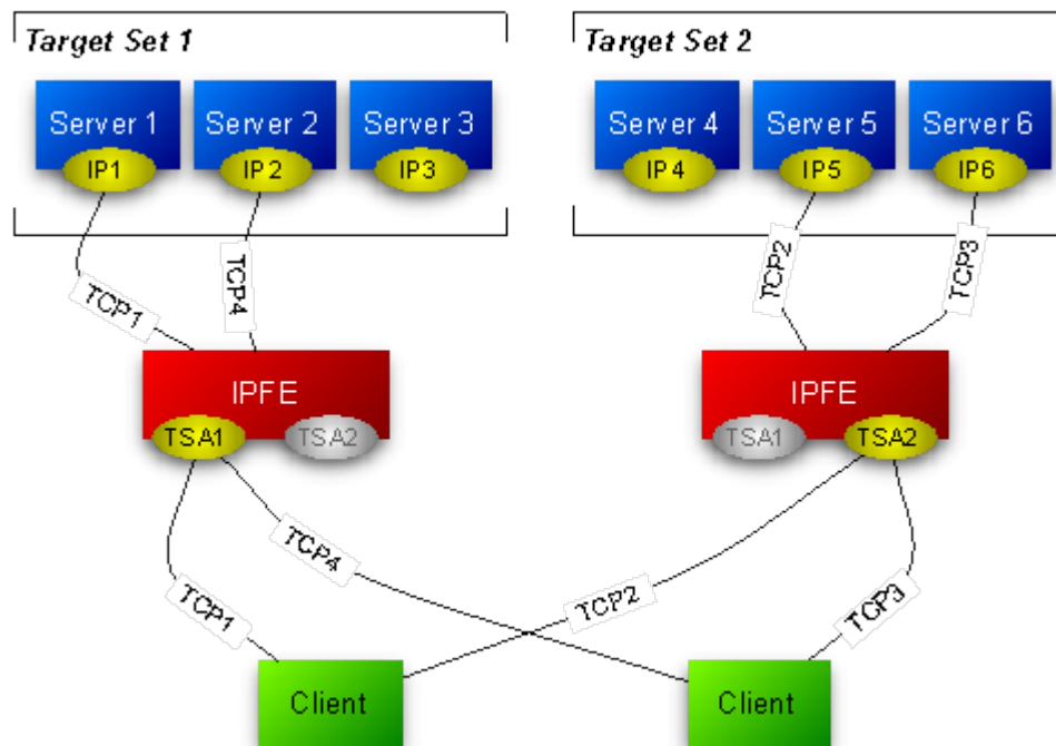
Figure 2-1 IPFE Architecture
